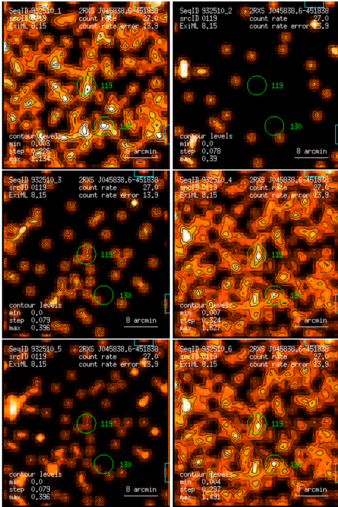
Figure 119: RASS 932510: detection 0119: band rate images, Gaussian filter: (1) PSPC channels 11 – 41, (2) 52 – 90, (3) 91 – 201, (4) 11 – 235, (5) 52 – 201, (6) 11 – 201. Broad band rates in counts/ks. Band rate contour levels in counts/ks/arcmin 2 .
