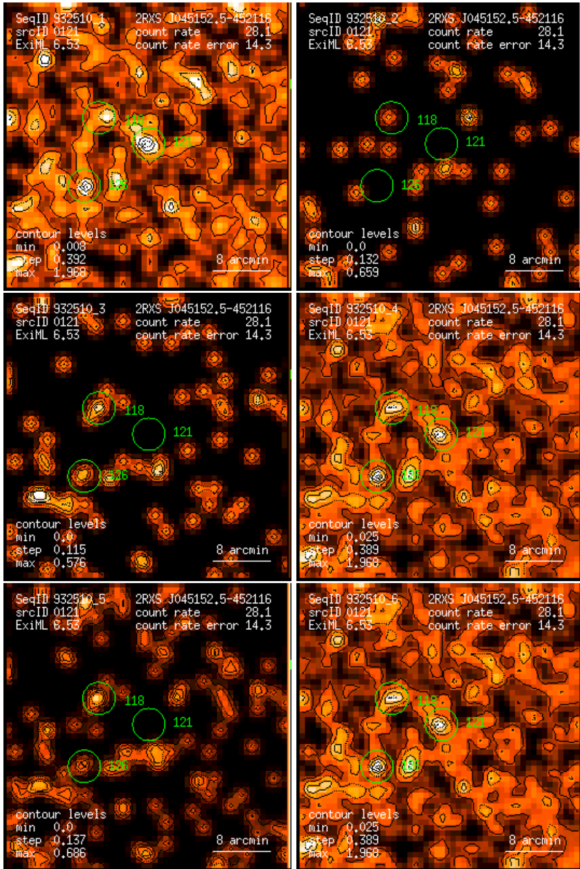
Figure 121: RASS 932510: detection 0121: band rate images, Gaussian filter: (1) PSPC channels 11 – 41, (2) 52 – 90, (3) 91 – 201, (4) 11 – 235, (5) 52 – 201, (6) 11 – 201. Broad band rates in counts/ks. Band rate contour levels in counts/ks/arcmin 2 .
