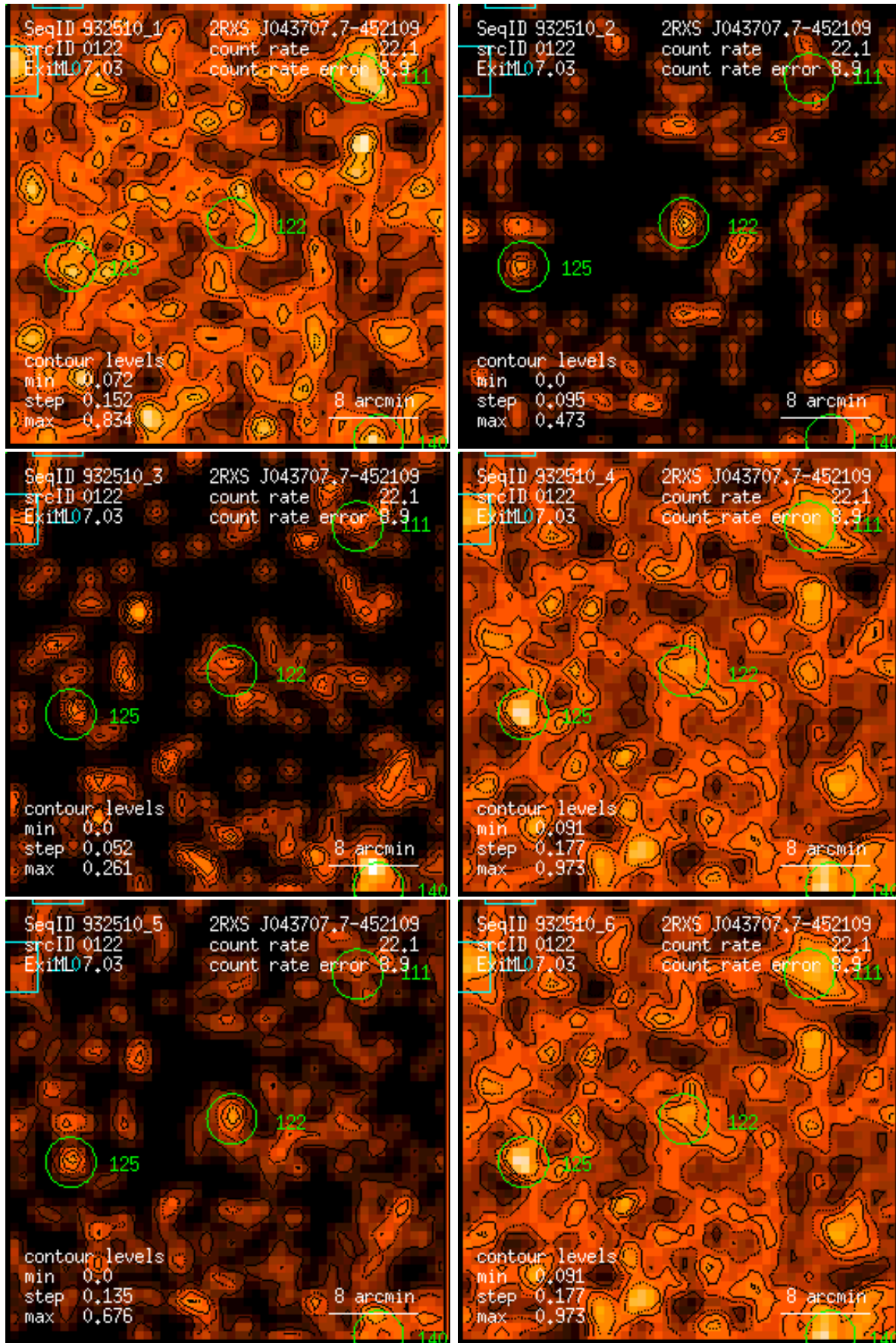
Figure 122: RASS 932510: detection 0122: band rate images, Gaussian filter: (1) PSPC channels 11 – 41, (2) 52 – 90, (3) 91 – 201, (4) 11 – 235, (5) 52 – 201, (6) 11 – 201. Broad band rates in counts/ks. Band rate contour levels in counts/ks/arcmin 2 .
