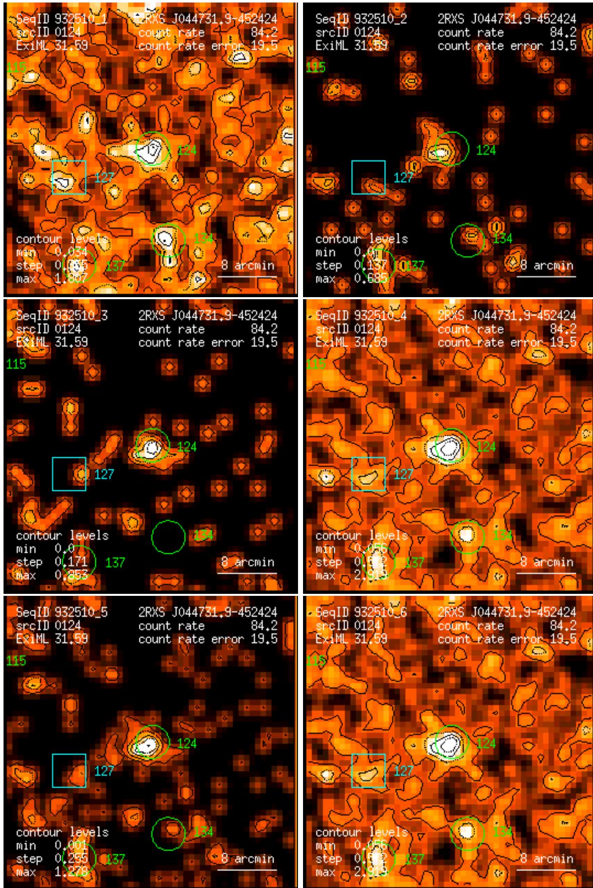
Figure 124: RASS 932510: detection 0124: band rate images, Gaussian filter: (1) PSPC channels 11 – 41, (2) 52 – 90, (3) 91 – 201, (4) 11 – 235, (5) 52 – 201, (6) 11 – 201. Broad band rates in counts/ks. Band rate contour levels in counts/ks/arcmin 2 .
