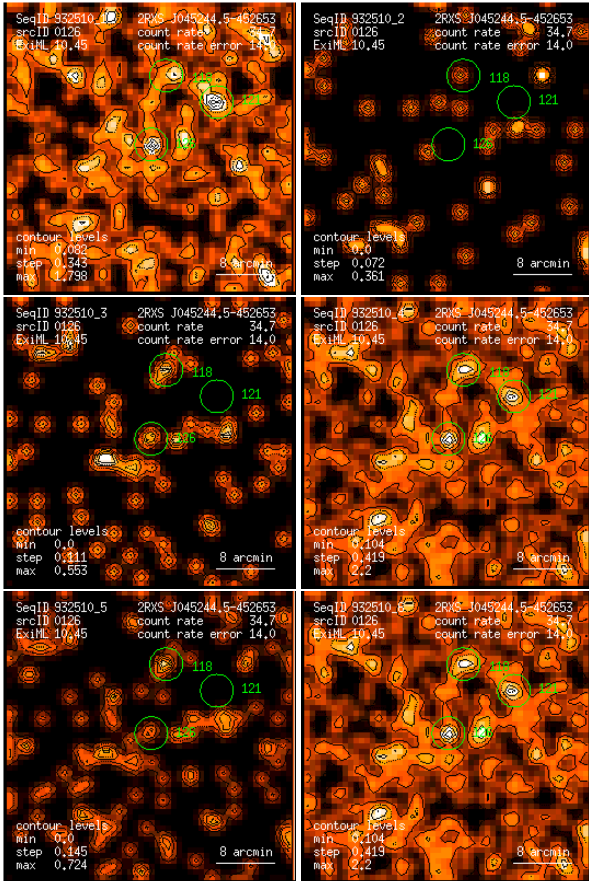
Figure 126: RASS 932510: detection 0126: band rate images, Gaussian filter: (1) PSPC channels 11 – 41, (2) 52 – 90, (3) 91 – 201, (4) 11 – 235, (5) 52 – 201, (6) 11 – 201. Broad band rates in counts/ks. Band rate contour levels in counts/ks/arcmin 2 .
