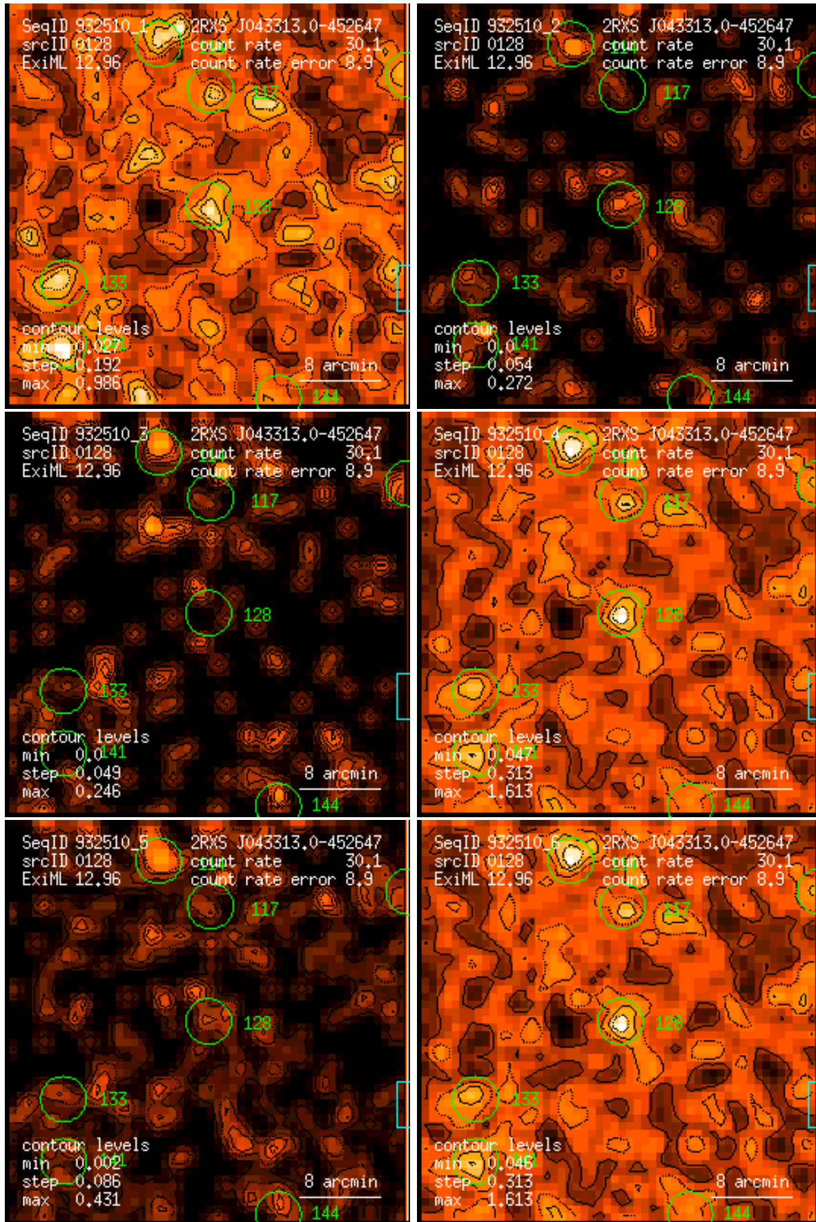
Figure 128: RASS 932510: detection 0128: band rate images, Gaussian filter: (1) PSPC channels 11 – 41, (2) 52 – 90, (3) 91 – 201, (4) 11 – 235, (5) 52 – 201, (6) 11 – 201. Broad band rates in counts/ks. Band rate contour levels in counts/ks/arcmin 2 .
