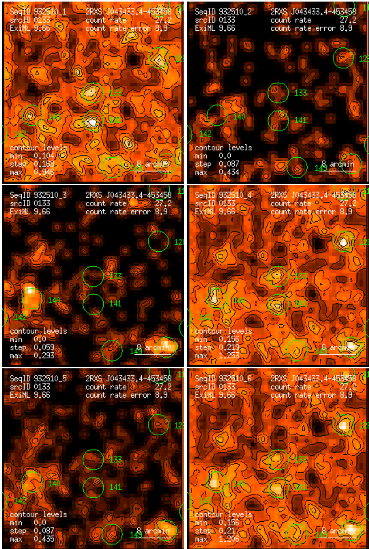
Figure 133: RASS 932510: detection 0133: band rate images, Gaussian filter: (1) PSPC channels 11 – 41, (2) 52 – 90, (3) 91 – 201, (4) 11 – 235, (5) 52 – 201, (6) 11 – 201. Broad band rates in counts/ks. Band rate contour levels in counts/ks/arcmin 2 .
