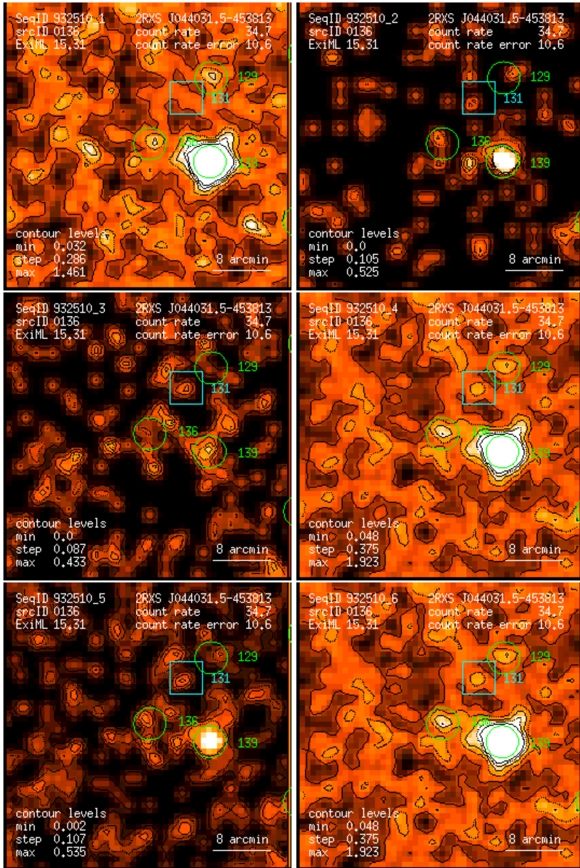
Figure 136: RASS 932510: detection 0136: band rate images, Gaussian filter: (1) PSPC channels 11 – 41, (2) 52 – 90, (3) 91 – 201, (4) 11 – 235, (5) 52 – 201, (6) 11 – 201. Broad band rates in counts/ks. Band rate contour levels in counts/ks/arcmin 2 .
