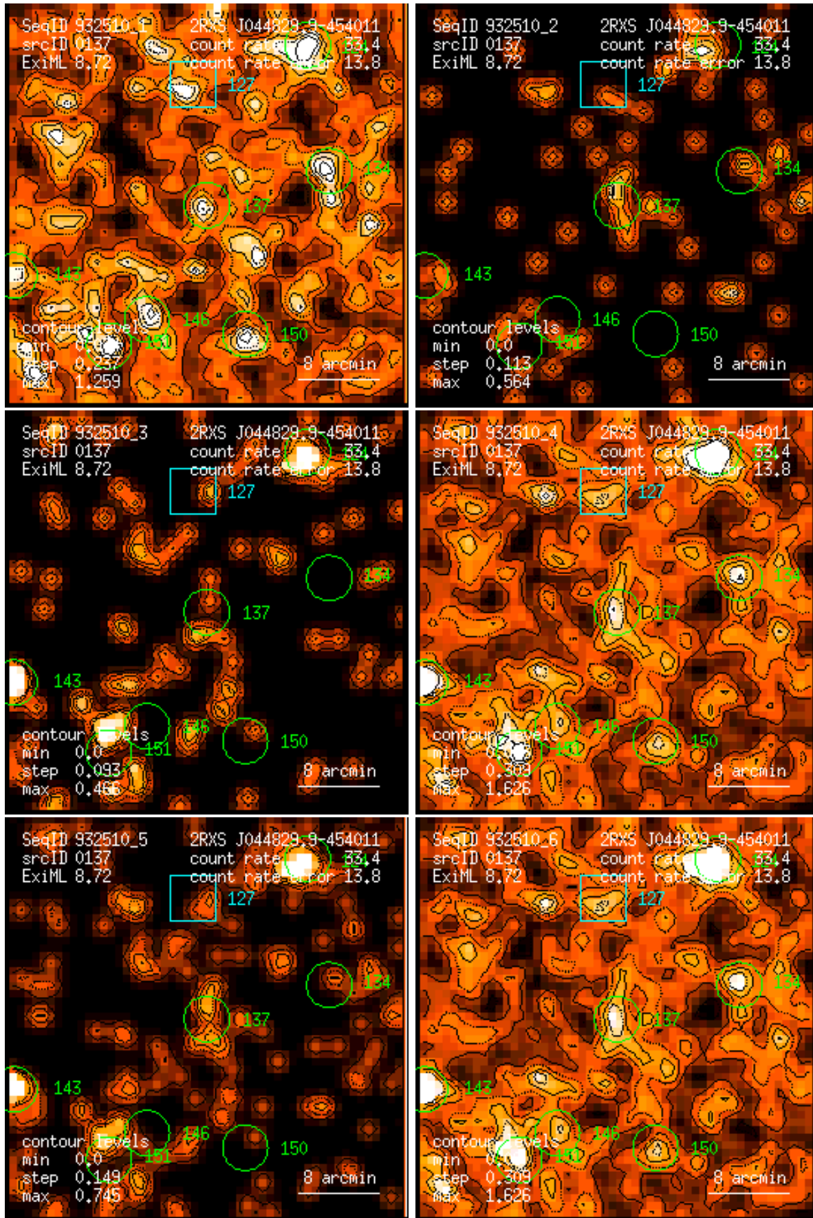
Figure 137: RASS 932510: detection 0137: band rate images, Gaussian filter: (1) PSPC channels 11 – 41, (2) 52 – 90, (3) 91 – 201, (4) 11 – 235, (5) 52 – 201, (6) 11 – 201. Broad band rates in counts/ks. Band rate contour levels in counts/ks/arcmin 2 .
