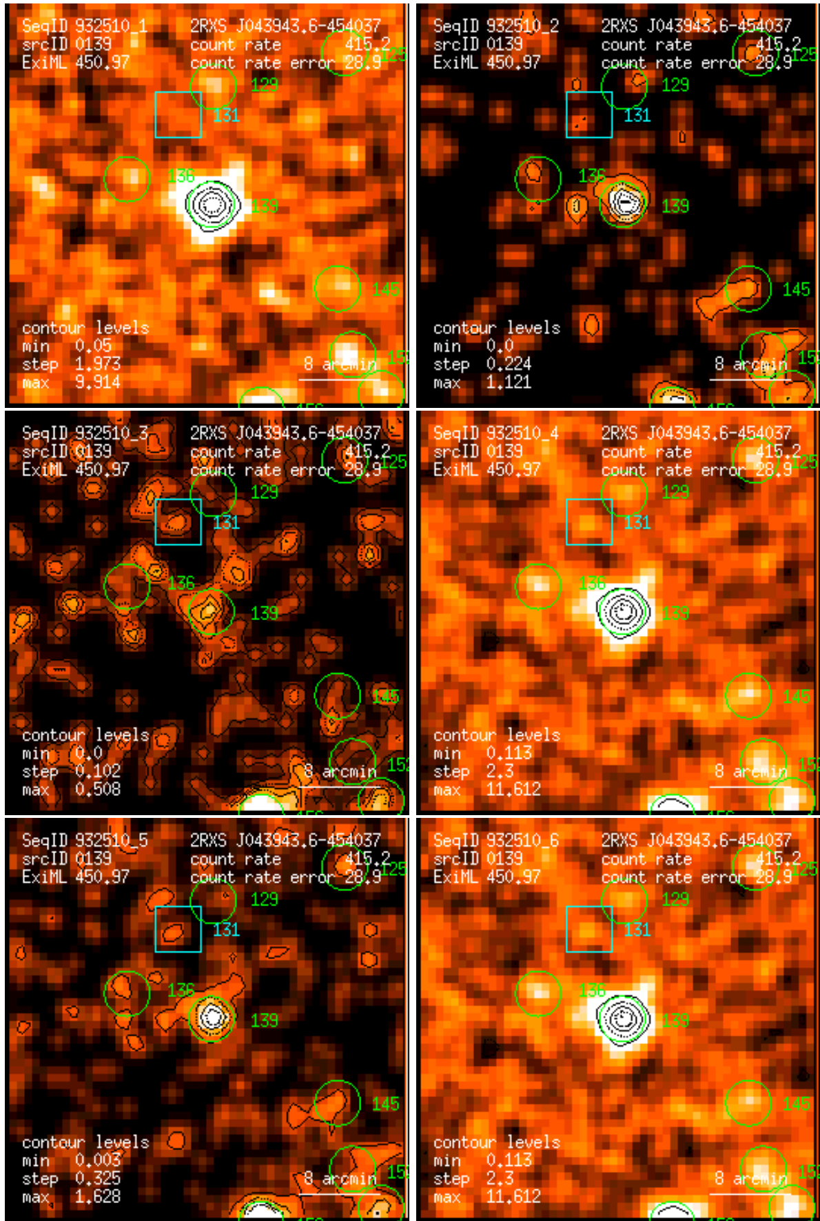
Figure 139: RASS 932510: detection 0139: band rate images, Gaussian filter: (1) PSPC channels 11 – 41, (2) 52 – 90, (3) 91 – 201, (4) 11 – 235, (5) 52 – 201, (6) 11 – 201. Broad band rates in counts/ks. Band rate contour levels in counts/ks/arcmin 2 .
