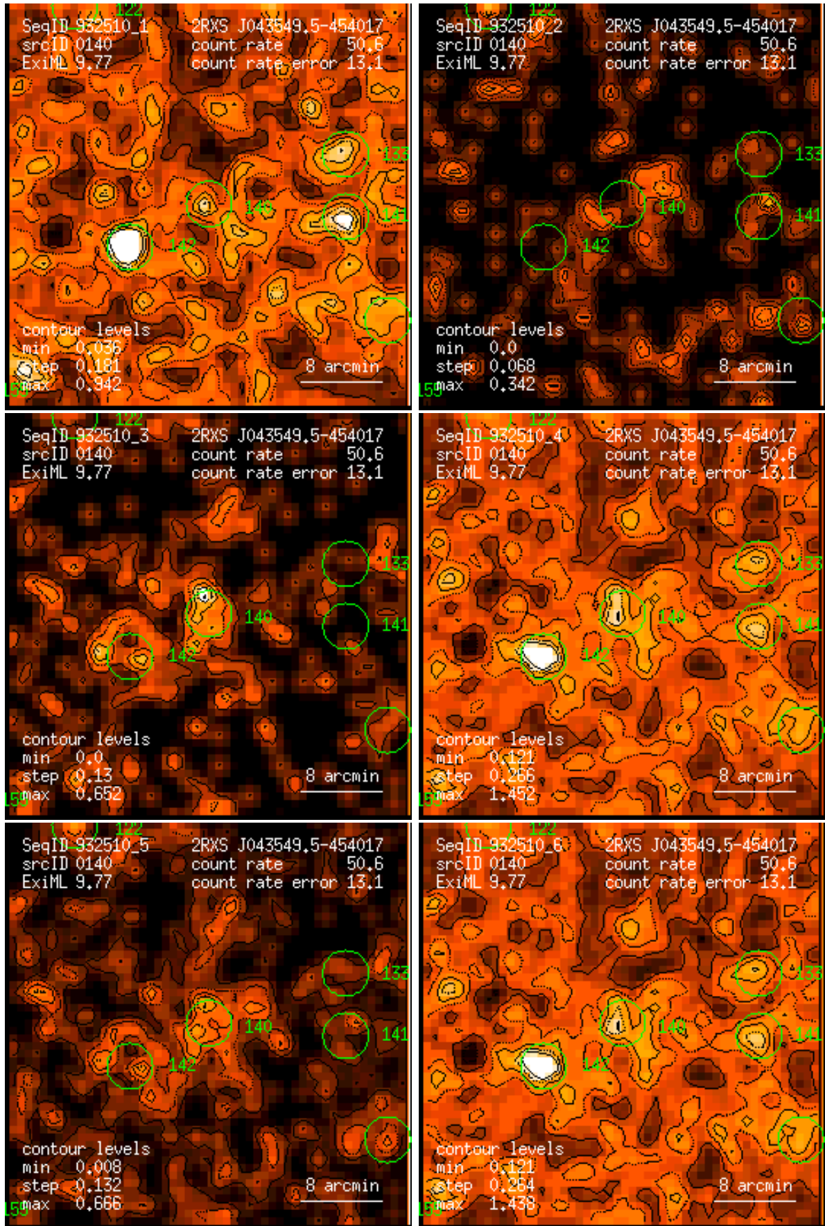
Figure 140: RASS 932510: detection 0140: band rate images, Gaussian filter: (1) PSPC channels 11 – 41, (2) 52 – 90, (3) 91 – 201, (4) 11 – 235, (5) 52 – 201, (6) 11 – 201. Broad band rates in counts/ks. Band rate contour levels in counts/ks/arcmin 2 .
