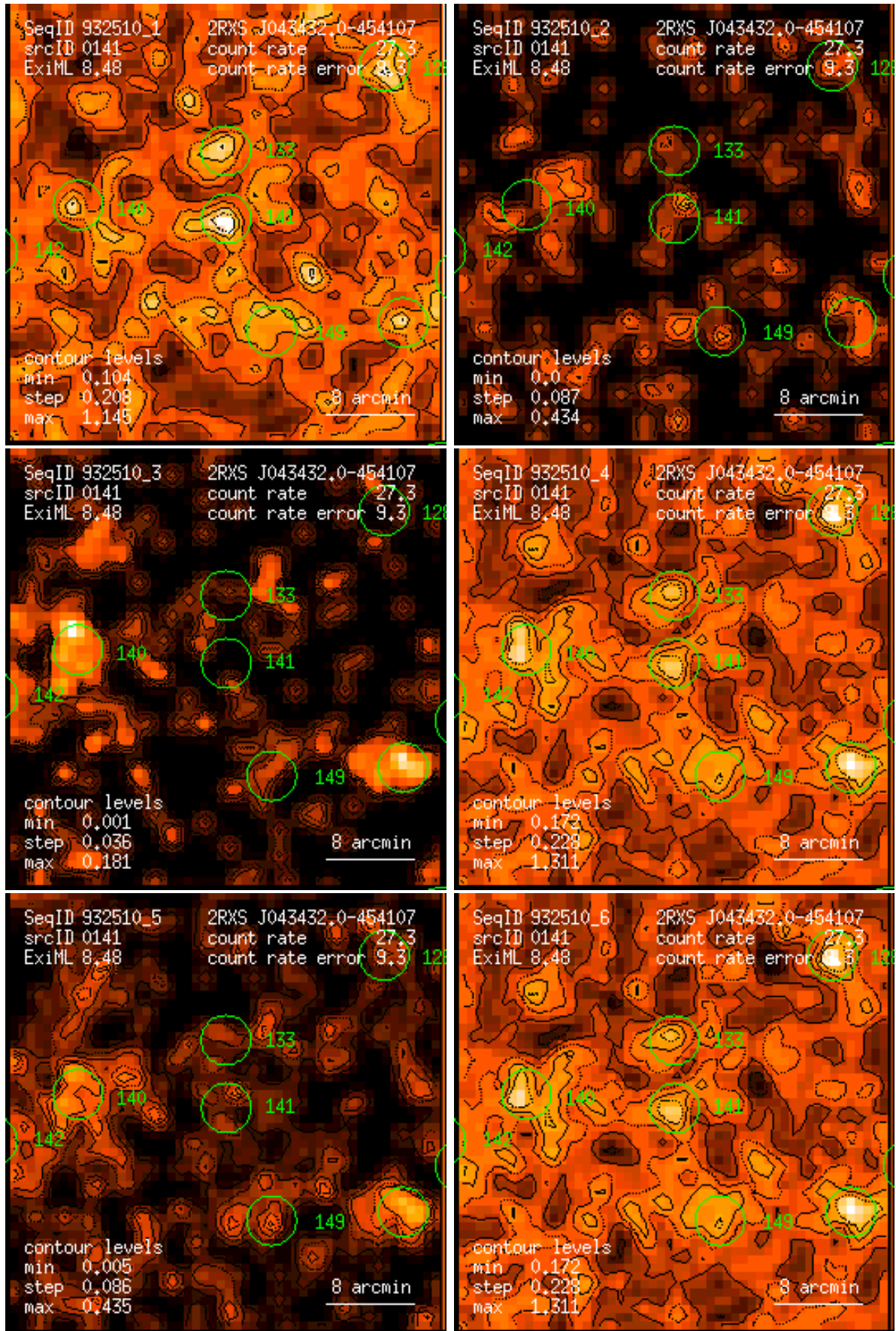
Figure 141: RASS 932510: detection 0141: band rate images, Gaussian filter: (1) PSPC channels 11 – 41, (2) 52 – 90, (3) 91 – 201, (4) 11 – 235, (5) 52 – 201, (6) 11 – 201. Broad band rates in counts/ks. Band rate contour levels in counts/ks/arcmin 2 .
