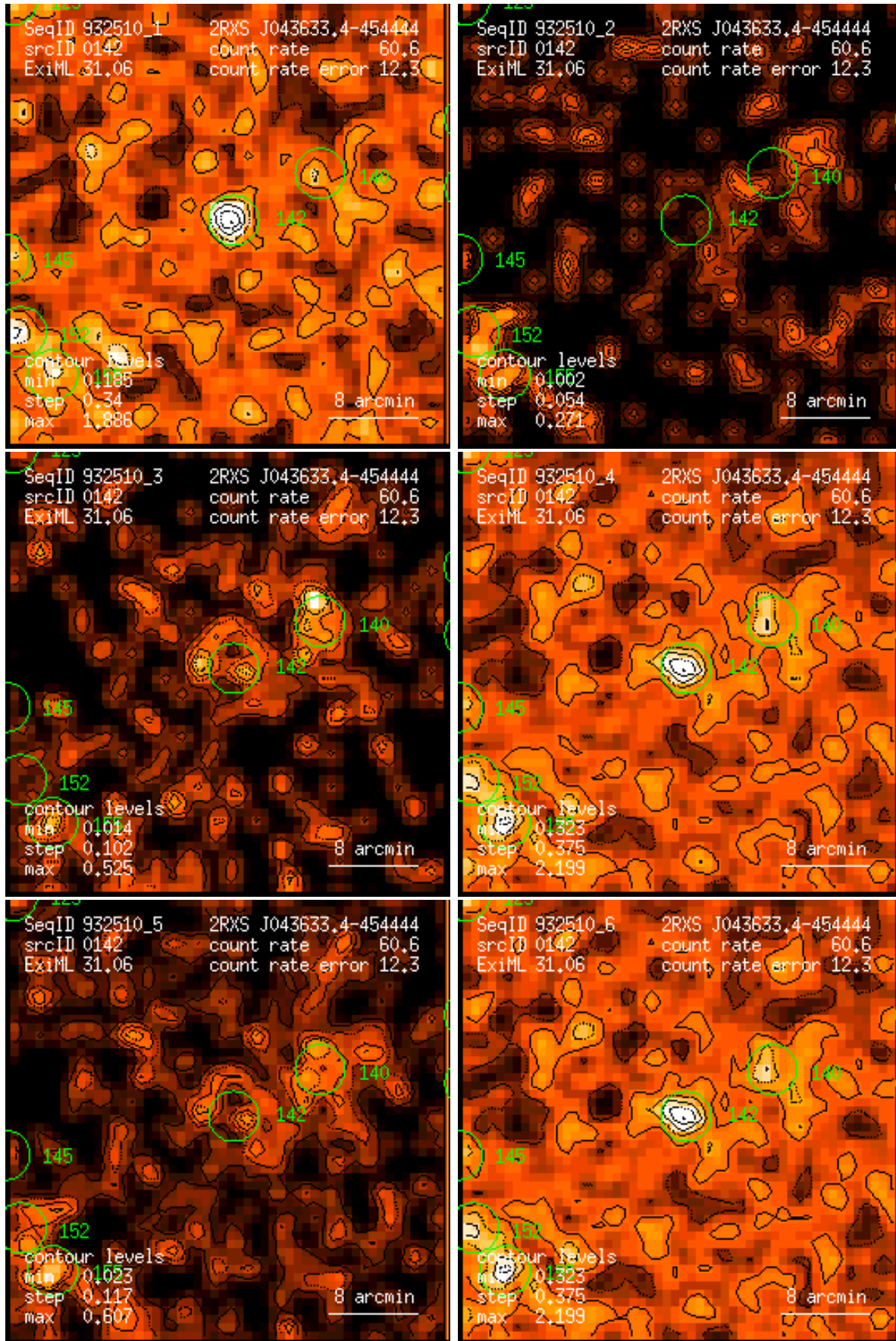
Figure 142: RASS 932510: detection 0142: band rate images, Gaussian filter: (1) PSPC channels 11 – 41, (2) 52 – 90, (3) 91 – 201, (4) 11 – 235, (5) 52 – 201, (6) 11 – 201. Broad band rates in counts/ks. Band rate contour levels in counts/ks/arcmin 2 .
