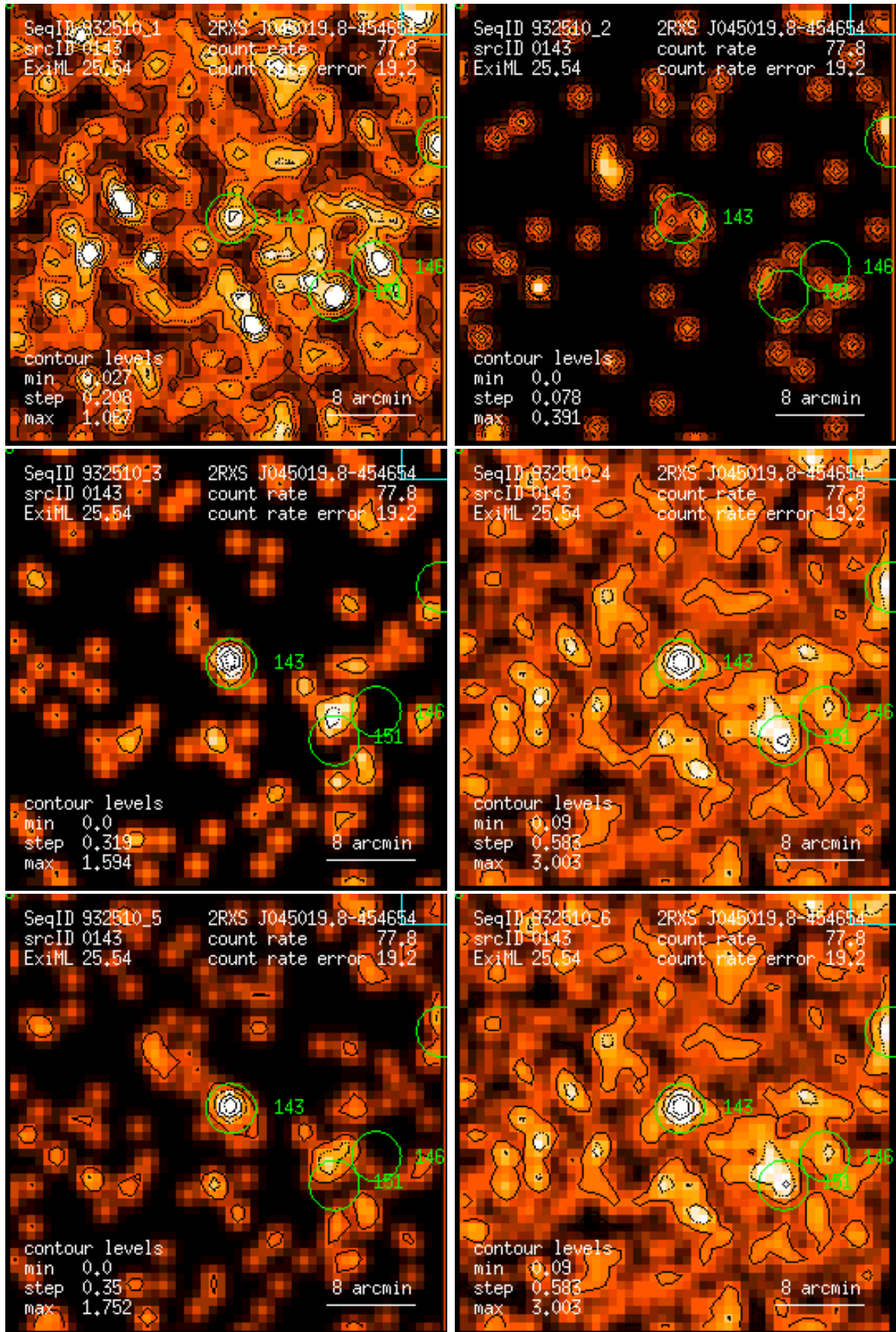
Figure 143: RASS 932510: detection 0143: band rate images, Gaussian filter: (1) PSPC channels 11 – 41, (2) 52 – 90, (3) 91 – 201, (4) 11 – 235, (5) 52 – 201, (6) 11 – 201. Broad band rates in counts/ks. Band rate contour levels in counts/ks/arcmin 2 .
