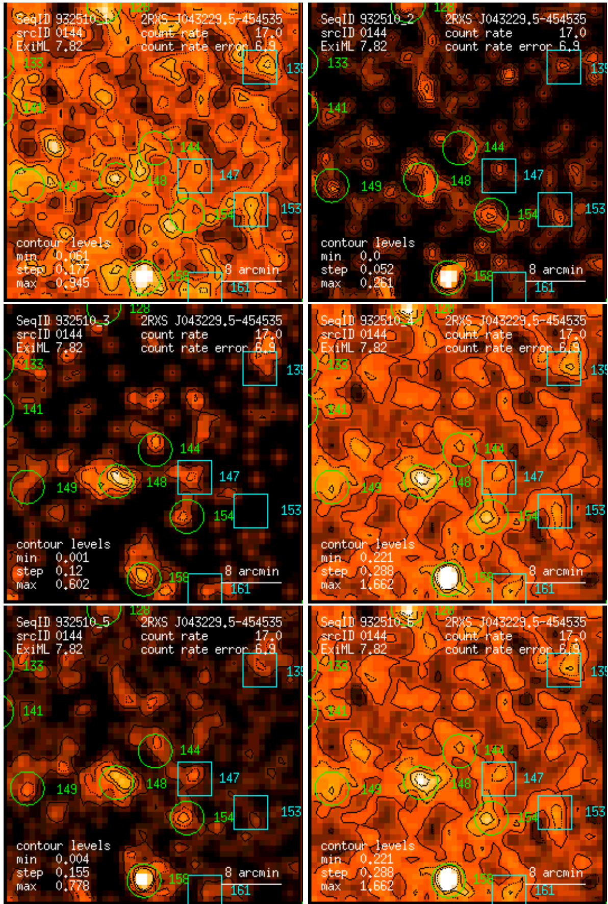
Figure 144: RASS 932510: detection 0144: band rate images, Gaussian filter: (1) PSPC channels 11 – 41, (2) 52 – 90, (3) 91 – 201, (4) 11 – 235, (5) 52 – 201, (6) 11 – 201. Broad band rates in counts/ks. Band rate contour levels in counts/ks/arcmin 2 .
