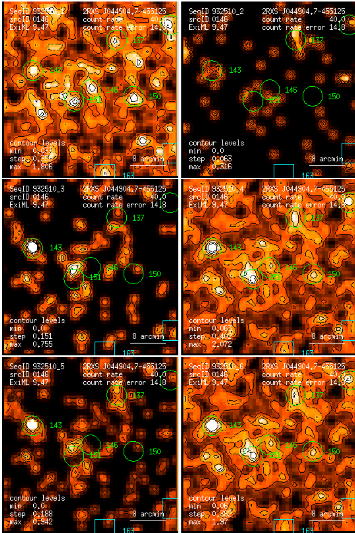
Figure 146: RASS 932510: detection 0146: band rate images, Gaussian filter: (1) PSPC channels 11 – 41, (2) 52 – 90, (3) 91 – 201, (4) 11 – 235, (5) 52 – 201, (6) 11 – 201. Broad band rates in counts/ks. Band rate contour levels in counts/ks/arcmin 2 .
