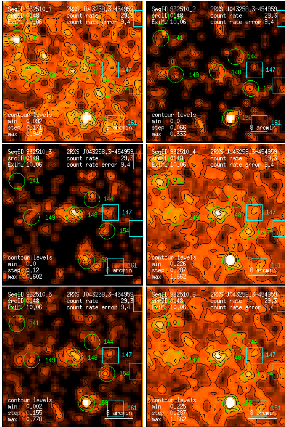
Figure 148: RASS 932510: detection 0148: band rate images, Gaussian filter: (1) PSPC channels 11 – 41, (2) 52 – 90, (3) 91 – 201, (4) 11 – 235, (5) 52 – 201, (6) 11 – 201. Broad band rates in counts/ks. Band rate contour levels in counts/ks/arcmin 2 .
