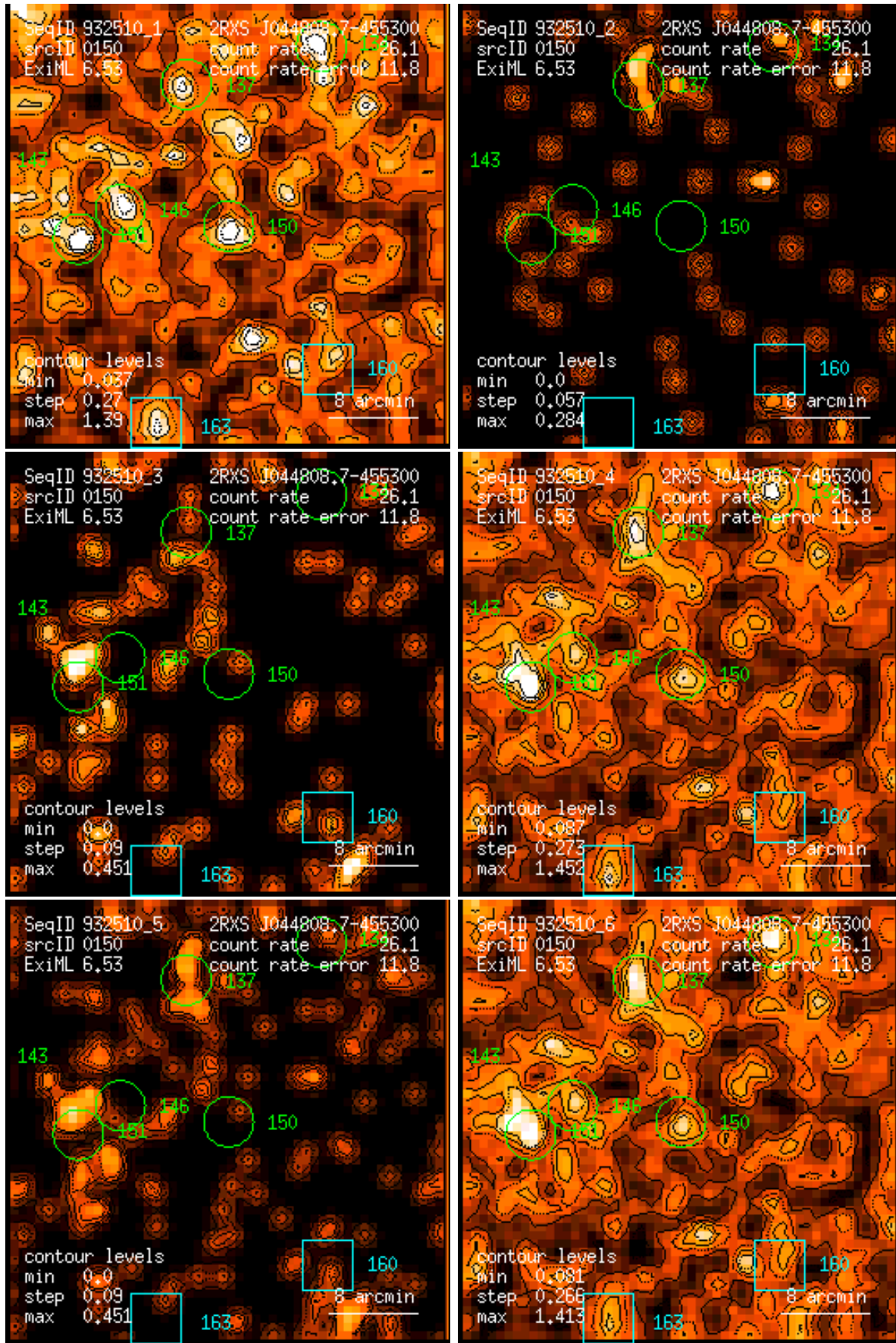
Figure 150: RASS 932510: detection 0150: band rate images, Gaussian filter: (1) PSPC channels 11 – 41, (2) 52 – 90, (3) 91 – 201, (4) 11 – 235, (5) 52 – 201, (6) 11 – 201. Broad band rates in counts/ks. Band rate contour levels in counts/ks/arcmin 2 .
