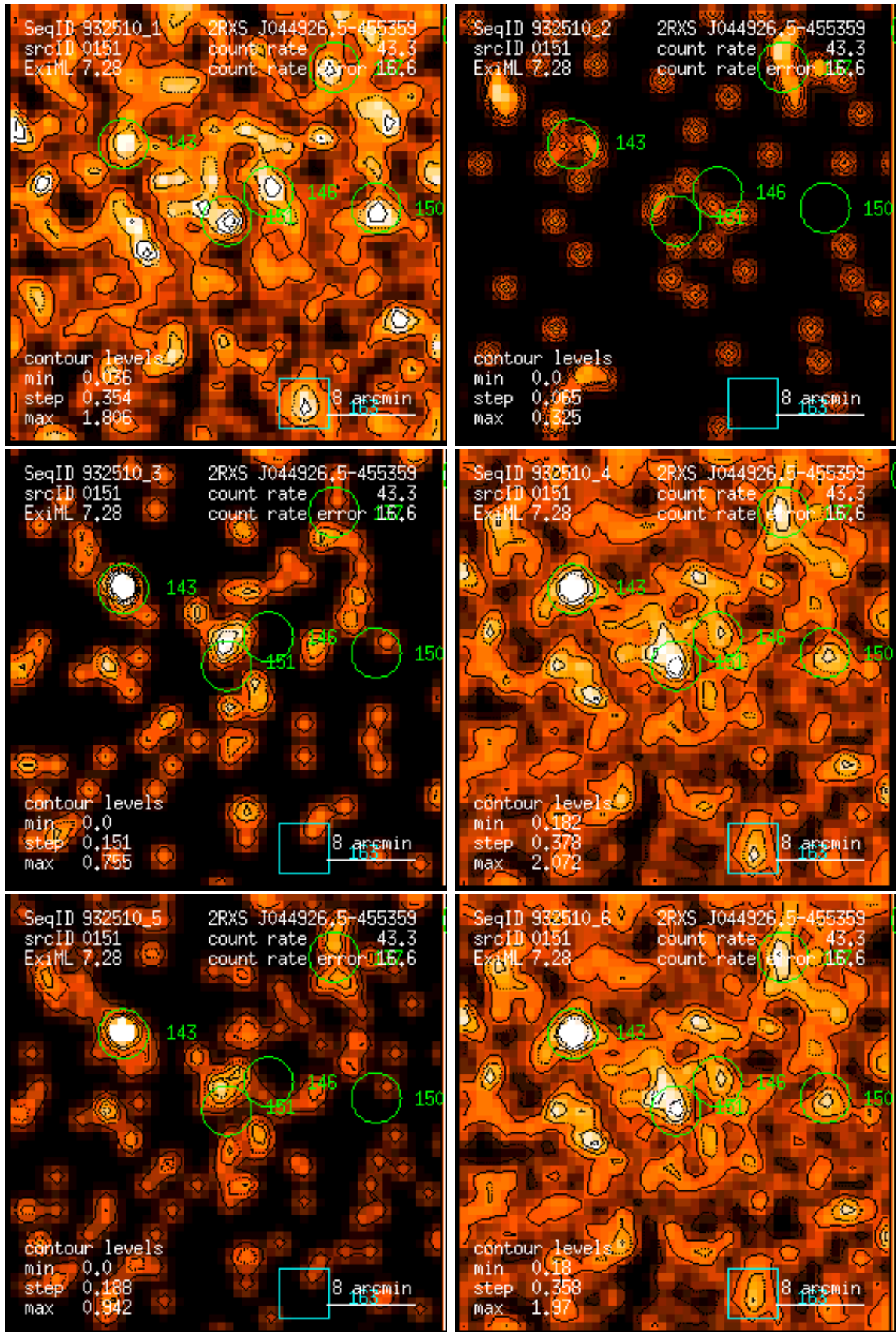
Figure 151: RASS 932510: detection 0151: band rate images, Gaussian filter: (1) PSPC channels 11 – 41, (2) 52 – 90, (3) 91 – 201, (4) 11 – 235, (5) 52 – 201, (6) 11 – 201. Broad band rates in counts/ks. Band rate contour levels in counts/ks/arcmin 2 .
