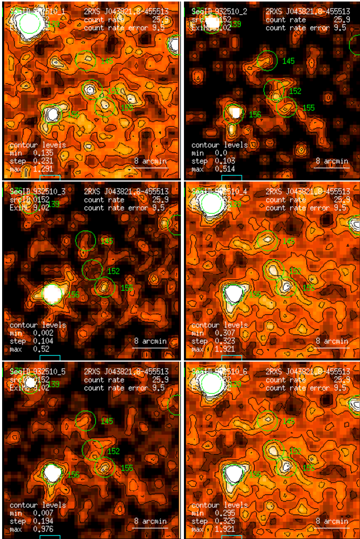
Figure 152: RASS 932510: detection 0152: band rate images, Gaussian filter: (1) PSPC channels 11 – 41, (2) 52 – 90, (3) 91 – 201, (4) 11 – 235, (5) 52 – 201, (6) 11 – 201. Broad band rates in counts/ks. Band rate contour levels in counts/ks/arcmin 2 .
