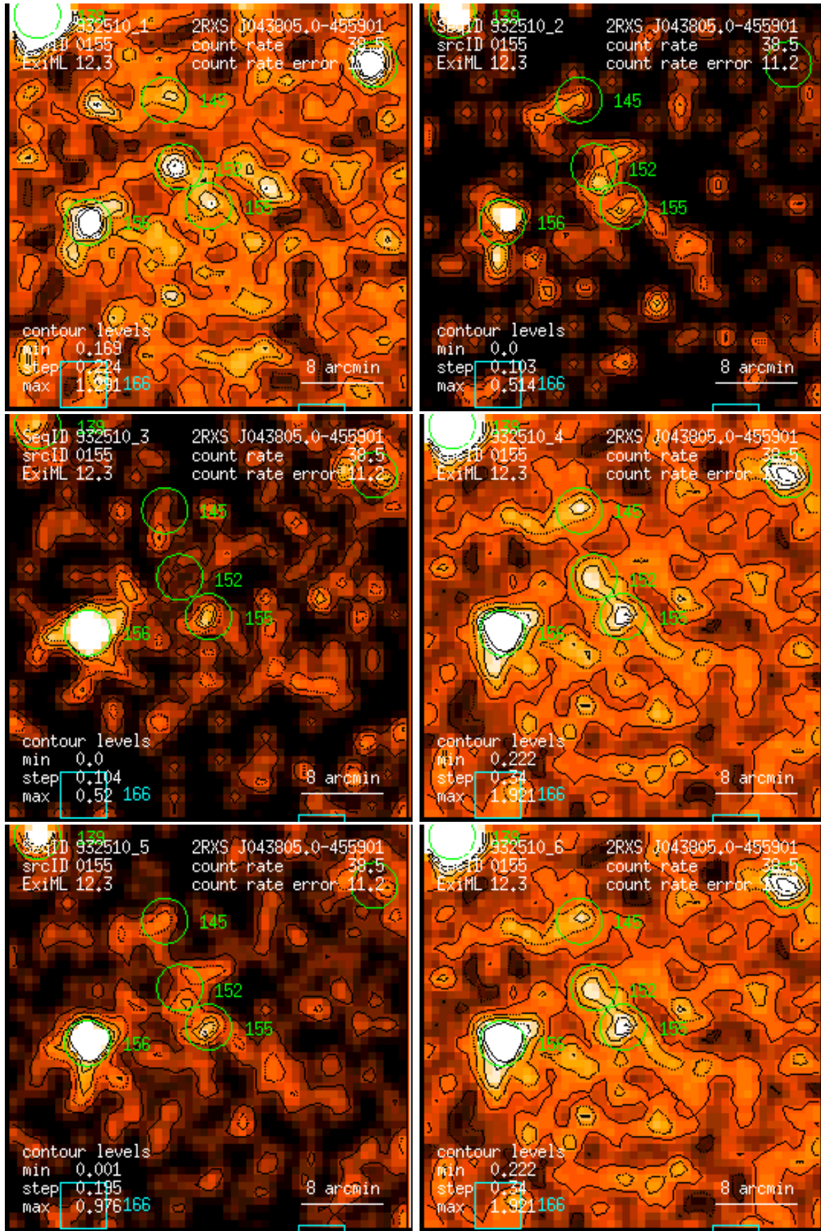
Figure 155: RASS 932510: detection 0155: band rate images, Gaussian filter: (1) PSPC channels 11 – 41, (2) 52 – 90, (3) 91 – 201, (4) 11 – 235, (5) 52 – 201, (6) 11 – 201. Broad band rates in counts/ks. Band rate contour levels in counts/ks/arcmin 2 .
