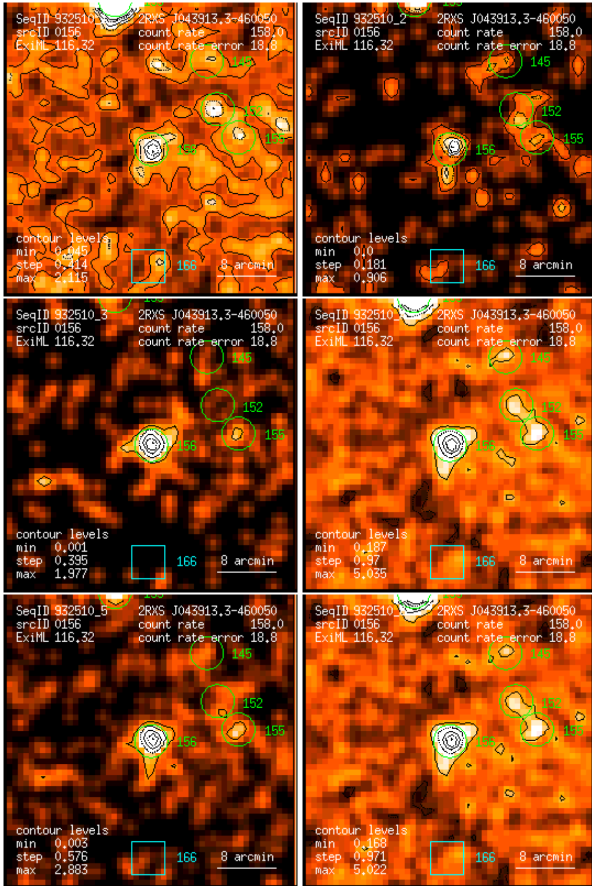
Figure 156: RASS 932510: detection 0156: band rate images, Gaussian filter: (1) PSPC channels 11 – 41, (2) 52 – 90, (3) 91 – 201, (4) 11 – 235, (5) 52 – 201, (6) 11 – 201. Broad band rates in counts/ks. Band rate contour levels in counts/ks/arcmin 2 .
