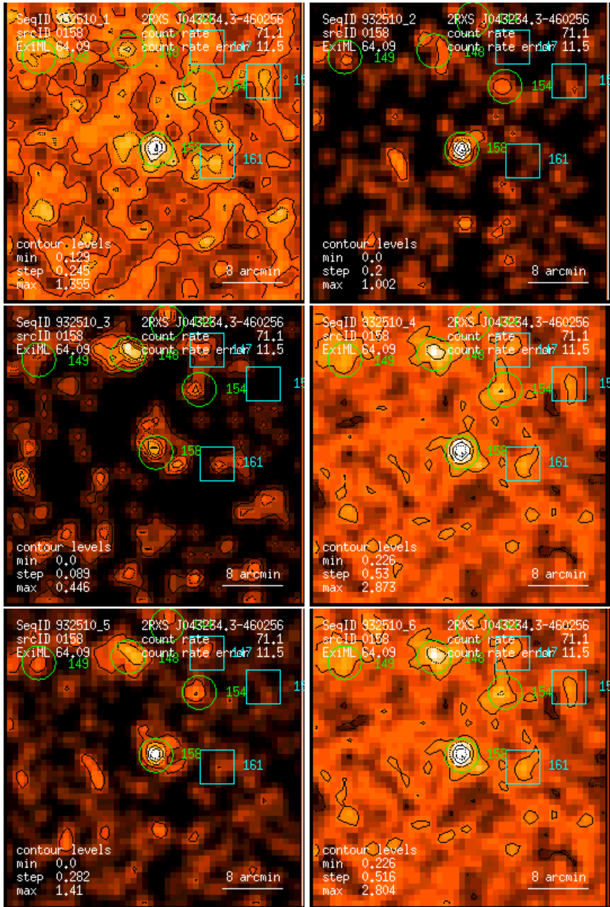
Figure 158: RASS 932510: detection 0158: band rate images, Gaussian filter: (1) PSPC channels 11 – 41, (2) 52 – 90, (3) 91 – 201, (4) 11 – 235, (5) 52 – 201, (6) 11 – 201. Broad band rates in counts/ks. Band rate contour levels in counts/ks/arcmin 2 .
