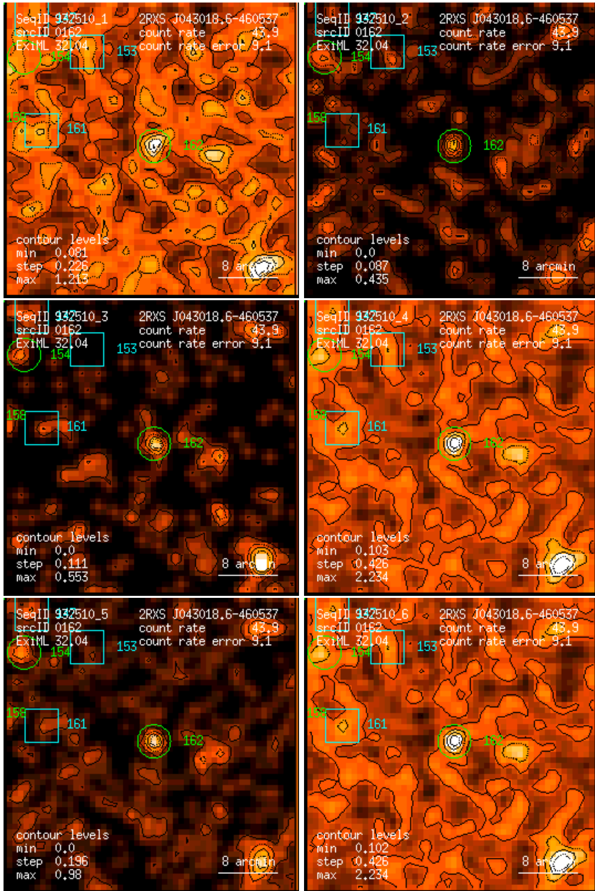
Figure 162: RASS 932510: detection 0162: band rate images, Gaussian filter: (1) PSPC channels 11 – 41, (2) 52 – 90, (3) 91 – 201, (4) 11 – 235, (5) 52 – 201, (6) 11 – 201. Broad band rates in counts/ks. Band rate contour levels in counts/ks/arcmin 2 .
