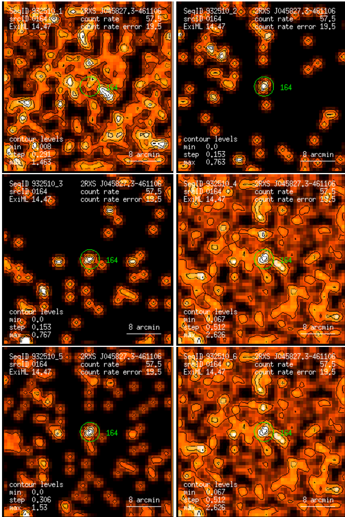
Figure 164: RASS 932510: detection 0164: band rate images, Gaussian filter: (1) PSPC channels 11 – 41, (2) 52 – 90, (3) 91 – 201, (4) 11 – 235, (5) 52 – 201, (6) 11 – 201. Broad band rates in counts/ks. Band rate contour levels in counts/ks/arcmin 2 .
