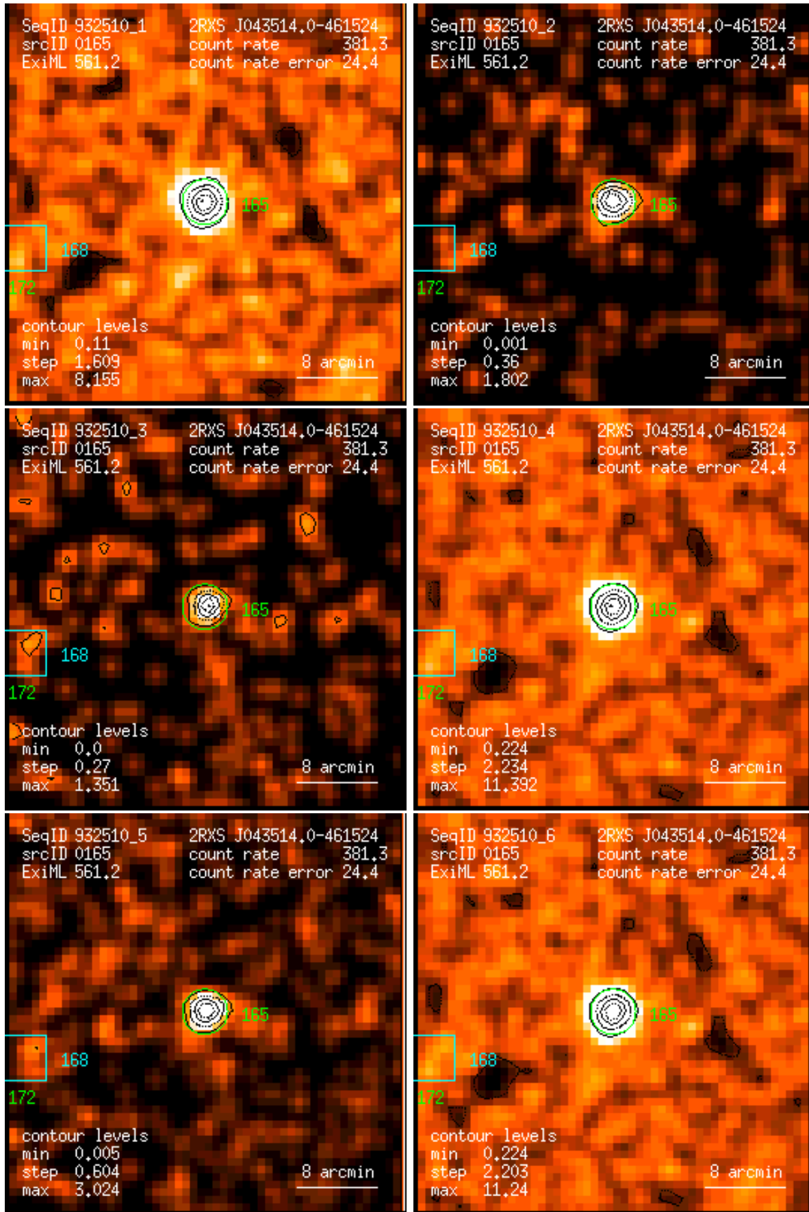
Figure 165: RASS 932510: detection 0165: band rate images, Gaussian filter: (1) PSPC channels 11 – 41, (2) 52 – 90, (3) 91 – 201, (4) 11 – 235, (5) 52 – 201, (6) 11 – 201. Broad band rates in counts/ks. Band rate contour levels in counts/ks/arcmin 2 .
