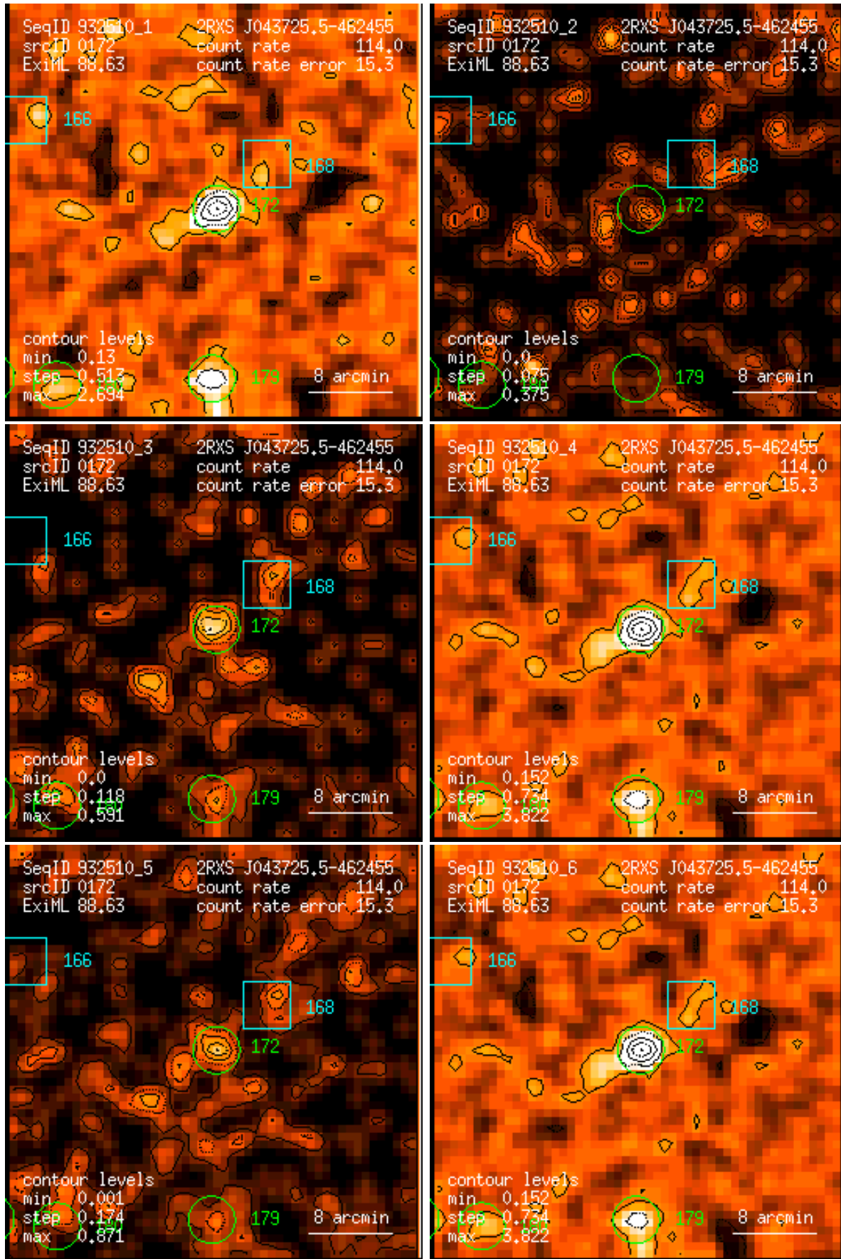
Figure 172: RASS 932510: detection 0172: band rate images, Gaussian filter: (1) PSPC channels 11 – 41, (2) 52 – 90, (3) 91 – 201, (4) 11 – 235, (5) 52 – 201, (6) 11 – 201. Broad band rates in counts/ks. Band rate contour levels in counts/ks/arcmin 2 .
