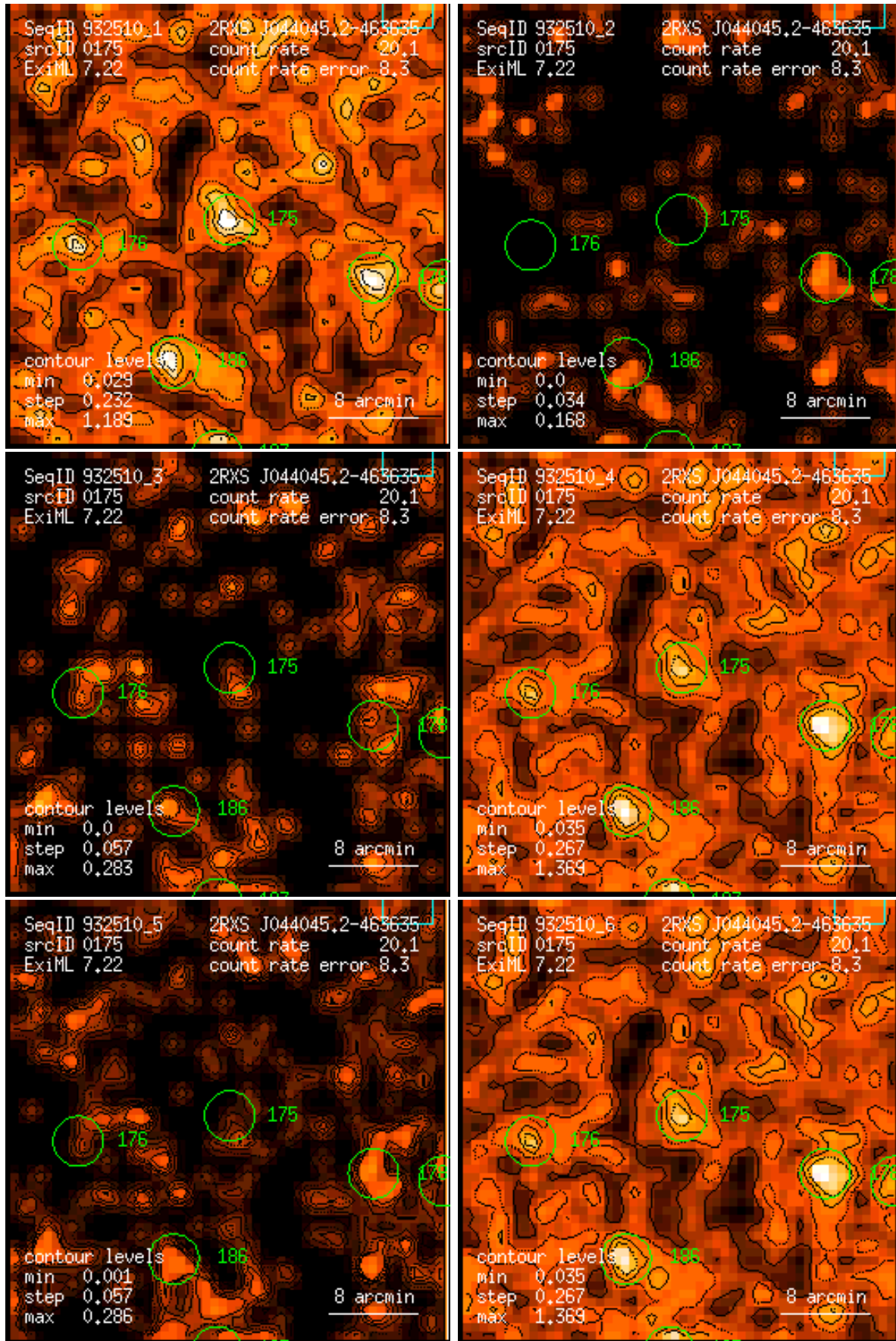
Figure 175: RASS 932510: detection 0175: band rate images, Gaussian filter: (1) PSPC channels 11 – 41, (2) 52 – 90, (3) 91 – 201, (4) 11 – 235, (5) 52 – 201, (6) 11 – 201. Broad band rates in counts/ks. Band rate contour levels in counts/ks/arcmin 2 .
