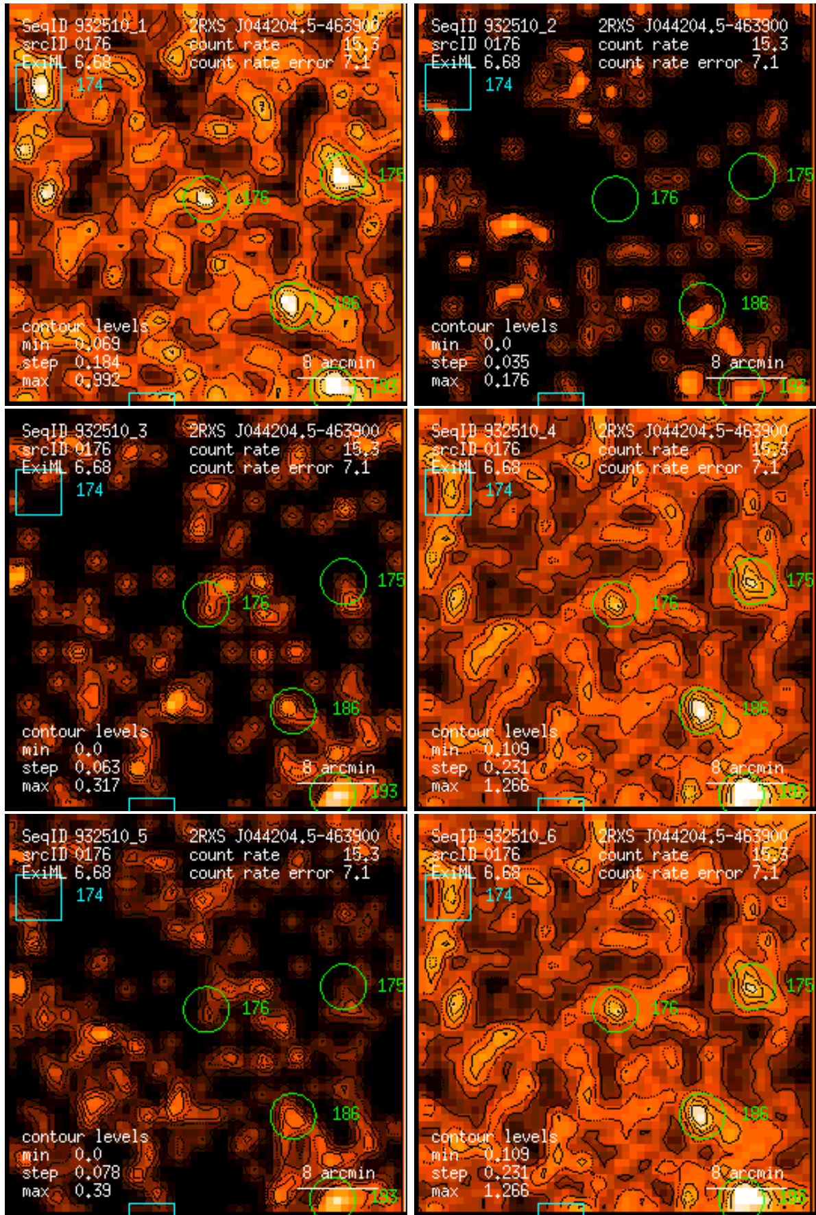
Figure 176: RASS 932510: detection 0176: band rate images, Gaussian filter: (1) PSPC channels 11 – 41, (2) 52 – 90, (3) 91 – 201, (4) 11 – 235, (5) 52 – 201, (6) 11 – 201. Broad band rates in counts/ks. Band rate contour levels in counts/ks/arcmin 2 .
