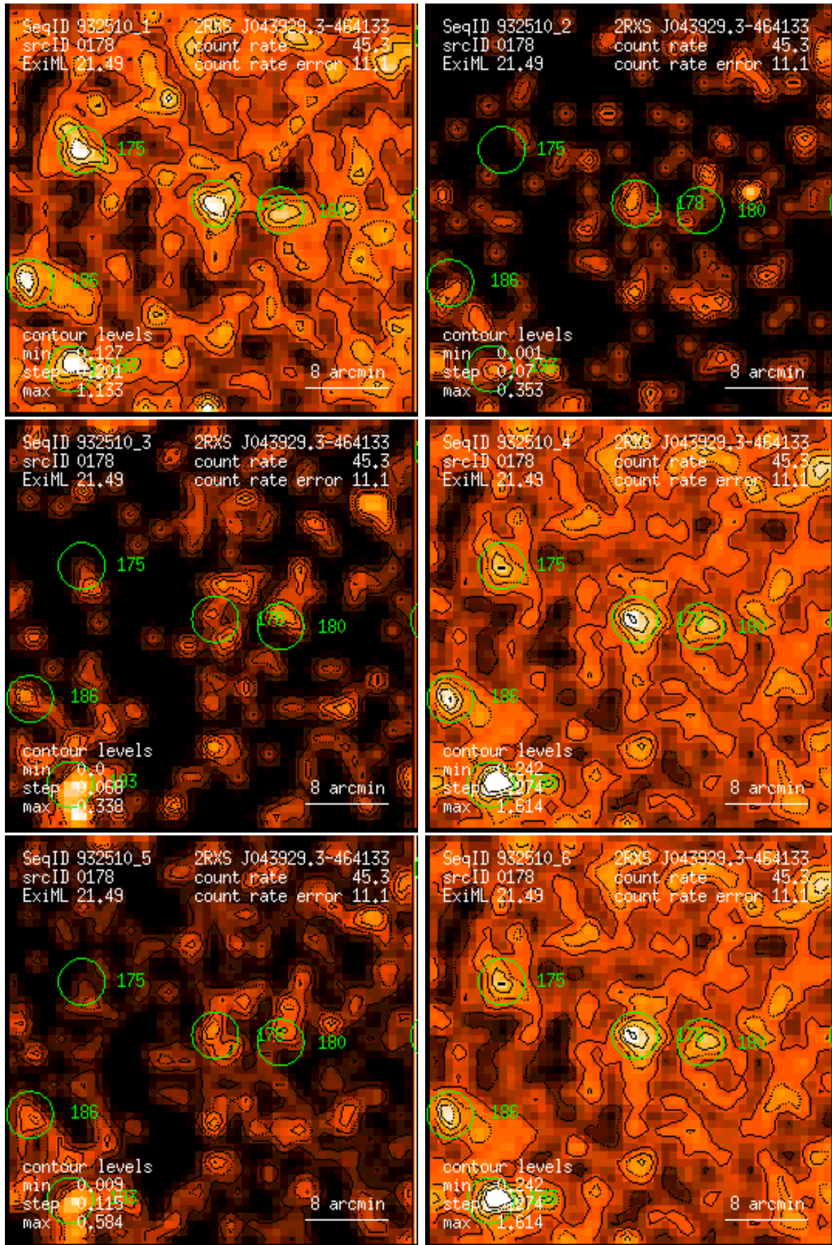
Figure 178: RASS 932510: detection 0178: band rate images, Gaussian filter: (1) PSPC channels 11 – 41, (2) 52 – 90, (3) 91 – 201, (4) 11 – 235, (5) 52 – 201, (6) 11 – 201. Broad band rates in counts/ks. Band rate contour levels in counts/ks/arcmin 2 .
