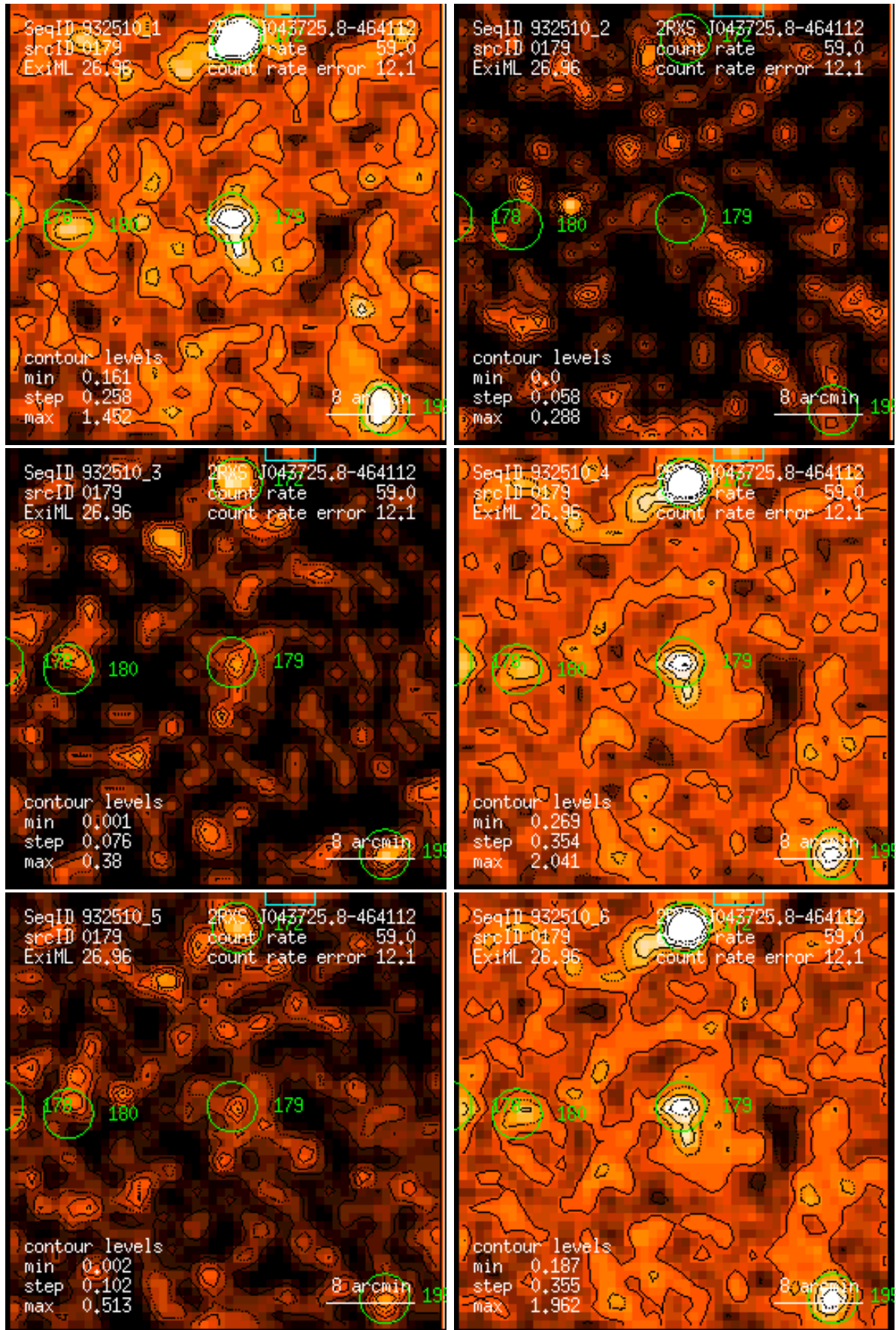
Figure 179: RASS 932510: detection 0179: band rate images, Gaussian filter: (1) PSPC channels 11 – 41, (2) 52 – 90, (3) 91 – 201, (4) 11 – 235, (5) 52 – 201, (6) 11 – 201. Broad band rates in counts/ks. Band rate contour levels in counts/ks/arcmin 2 .
