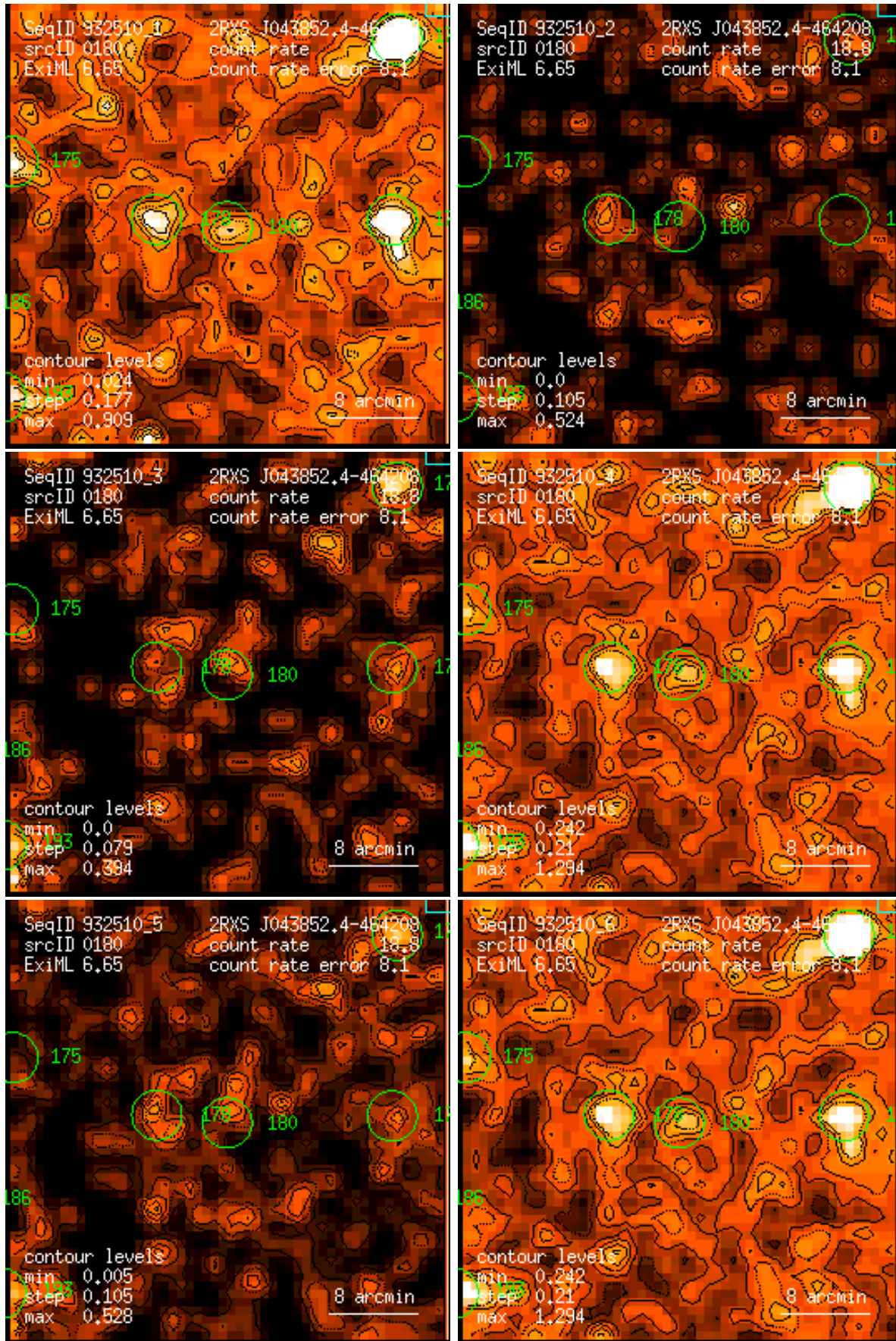
Figure 180: RASS 932510: detection 0180: band rate images, Gaussian filter: (1) PSPC channels 11 – 41, (2) 52 – 90, (3) 91 – 201, (4) 11 – 235, (5) 52 – 201, (6) 11 – 201. Broad band rates in counts/ks. Band rate contour levels in counts/ks/arcmin 2 .
