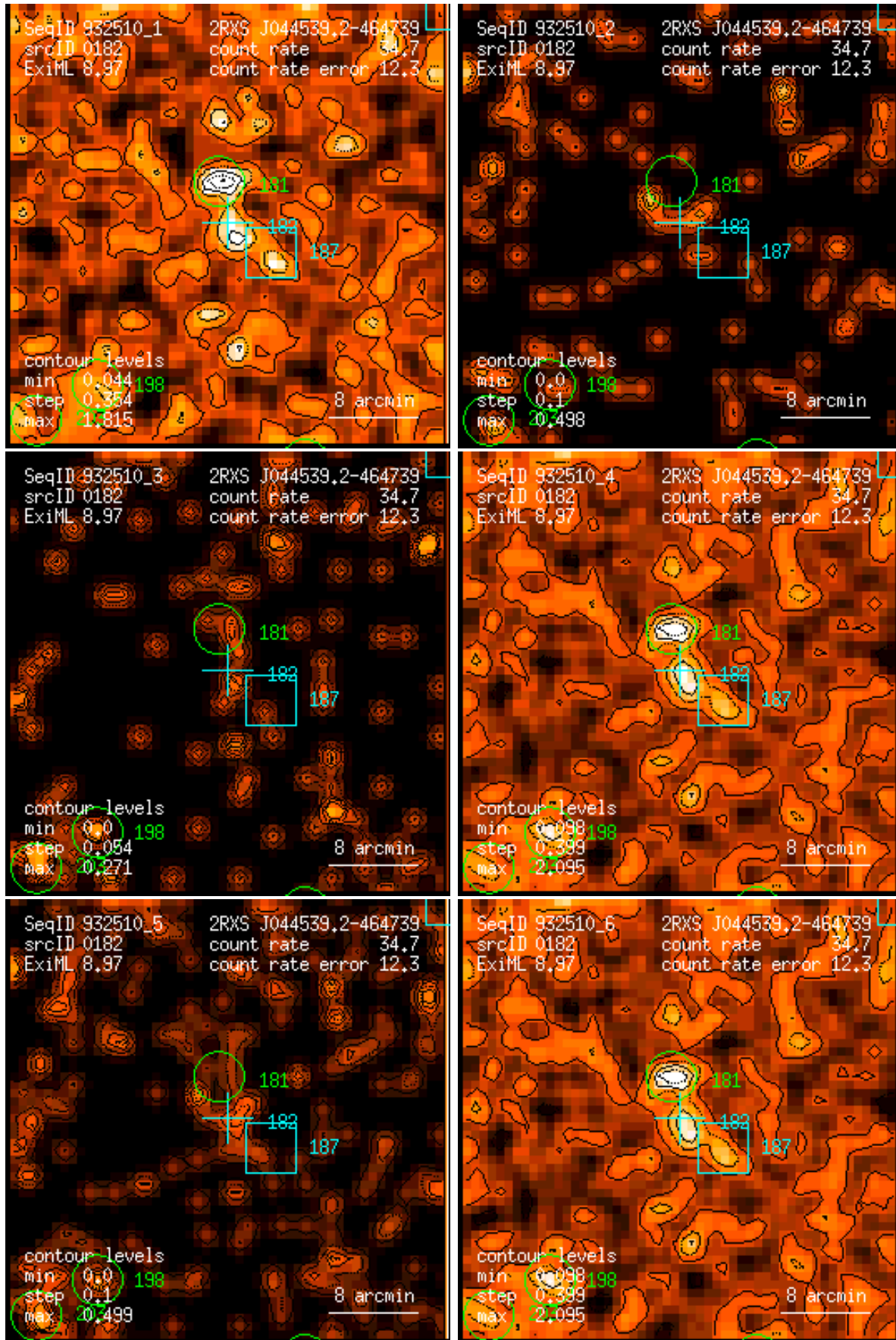
Figure 182: RASS 932510: detection 0182: band rate images, Gaussian filter: (1) PSPC channels 11 – 41, (2) 52 – 90, (3) 91 – 201, (4) 11 – 235, (5) 52 – 201, (6) 11 – 201. Broad band rates in counts/ks. Band rate contour levels in counts/ks/arcmin 2 .
