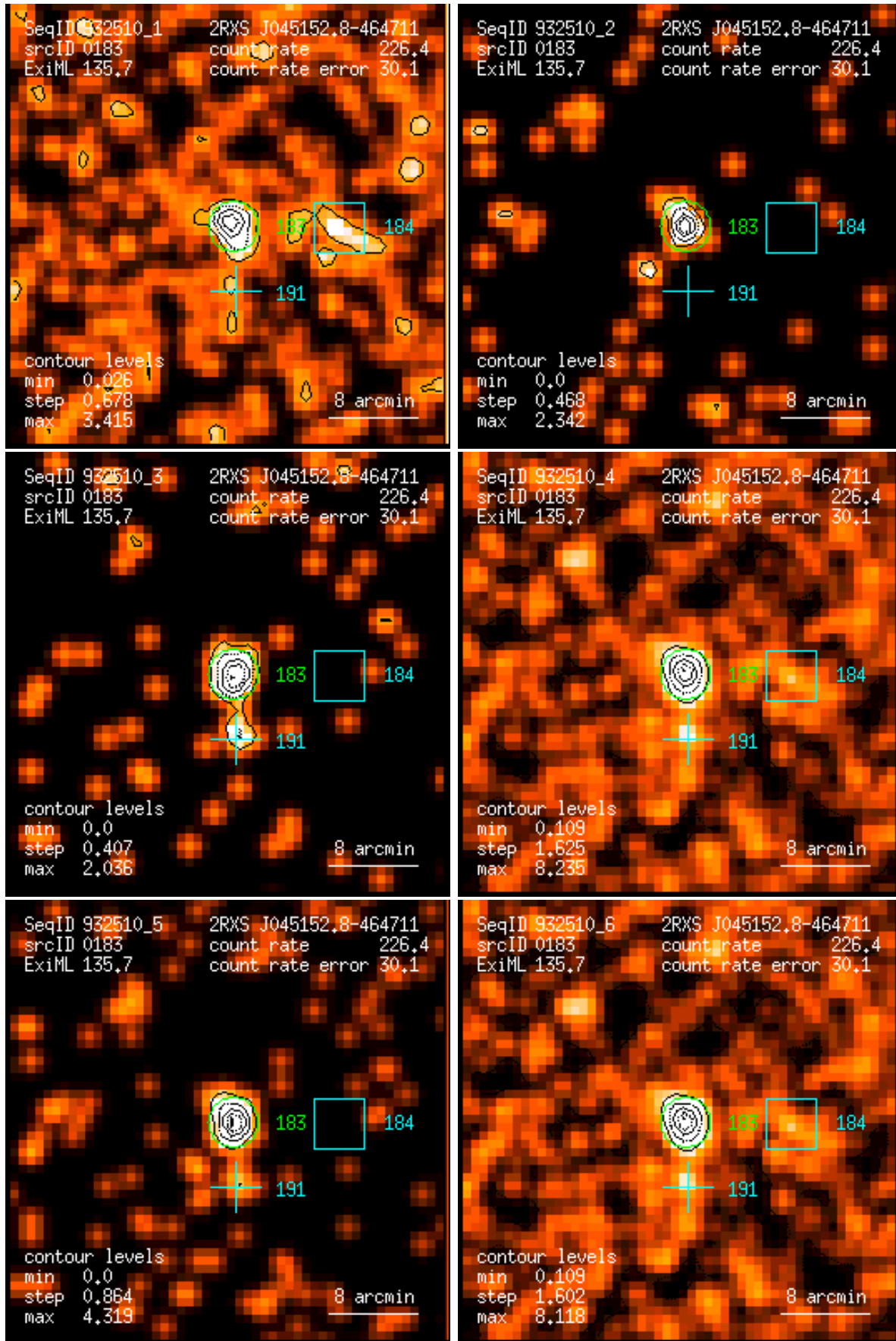
Figure 183: RASS 932510: detection 0183: band rate images, Gaussian filter: (1) PSPC channels 11 – 41, (2) 52 – 90, (3) 91 – 201, (4) 11 – 235, (5) 52 – 201, (6) 11 – 201. Broad band rates in counts/ks. Band rate contour levels in counts/ks/arcmin 2 .
