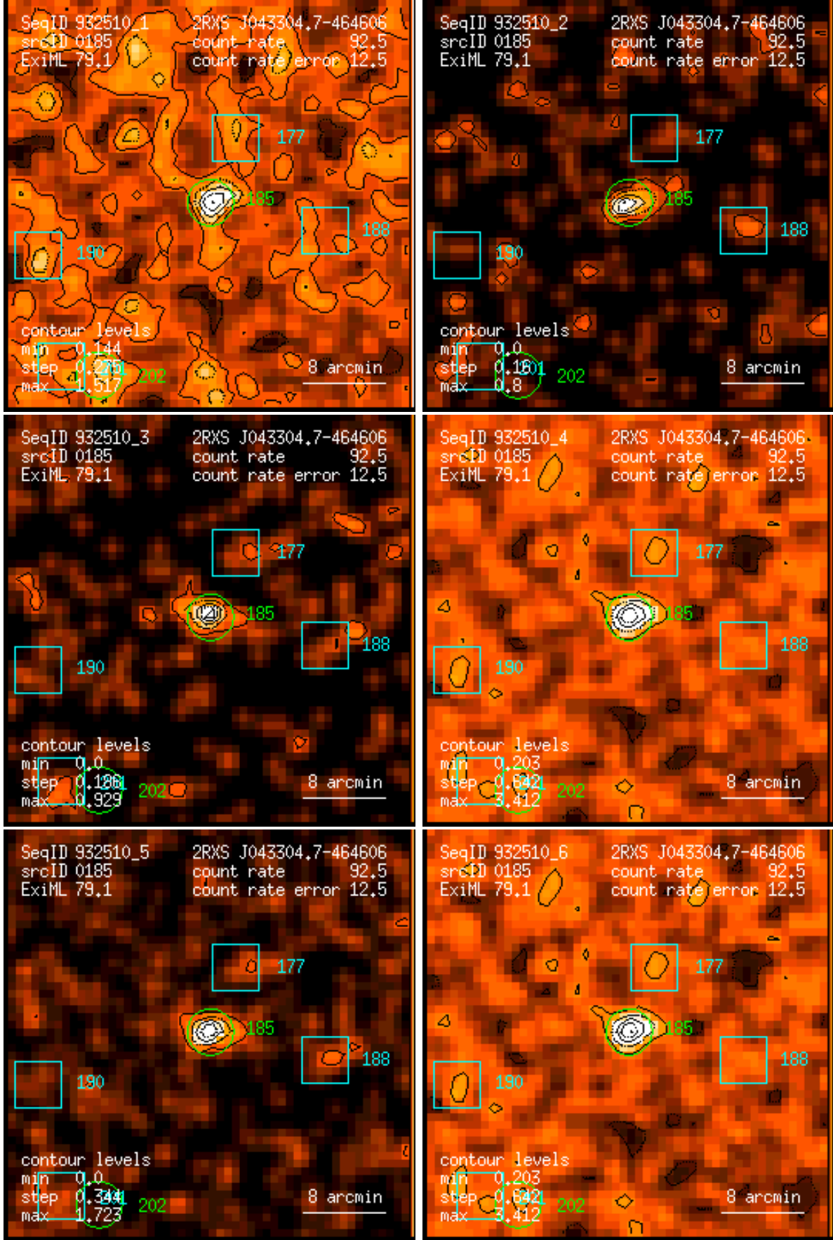
Figure 185: RASS 932510: detection 0185: band rate images, Gaussian filter: (1) PSPC channels 11 – 41, (2) 52 – 90, (3) 91 – 201, (4) 11 – 235, (5) 52 – 201, (6) 11 – 201. Broad band rates in counts/ks. Band rate contour levels in counts/ks/arcmin 2 .
