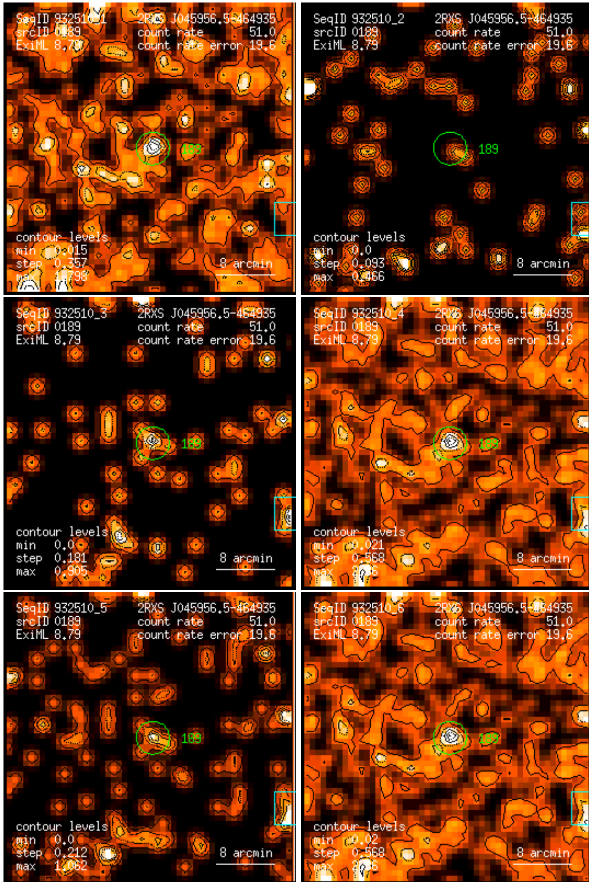
Figure 189: RASS 932510: detection 0189: band rate images, Gaussian filter: (1) PSPC channels 11 – 41, (2) 52 – 90, (3) 91 – 201, (4) 11 – 235, (5) 52 – 201, (6) 11 – 201. Broad band rates in counts/ks. Band rate contour levels in counts/ks/arcmin 2 .
