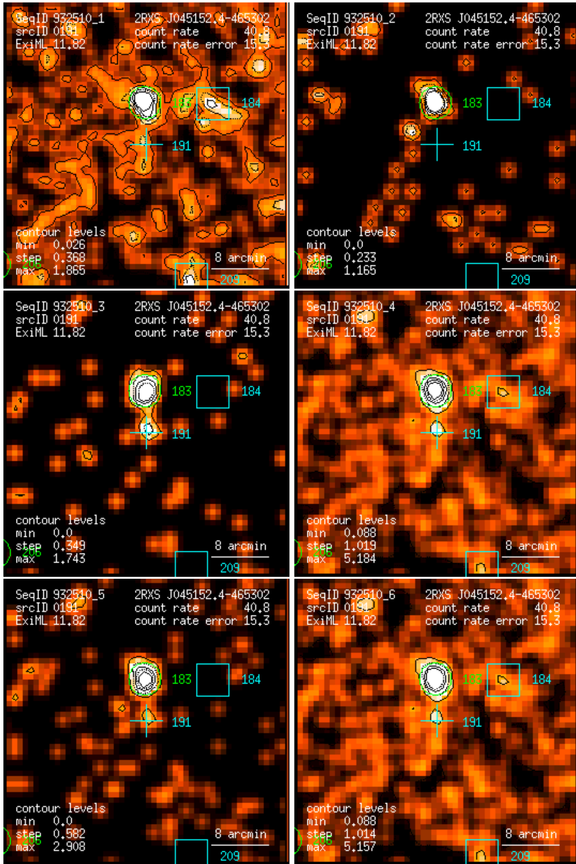
Figure 191: RASS 932510: detection 0191: band rate images, Gaussian filter: (1) PSPC channels 11 – 41, (2) 52 – 90, (3) 91 – 201, (4) 11 – 235, (5) 52 – 201, (6) 11 – 201. Broad band rates in counts/ks. Band rate contour levels in counts/ks/arcmin 2 .
