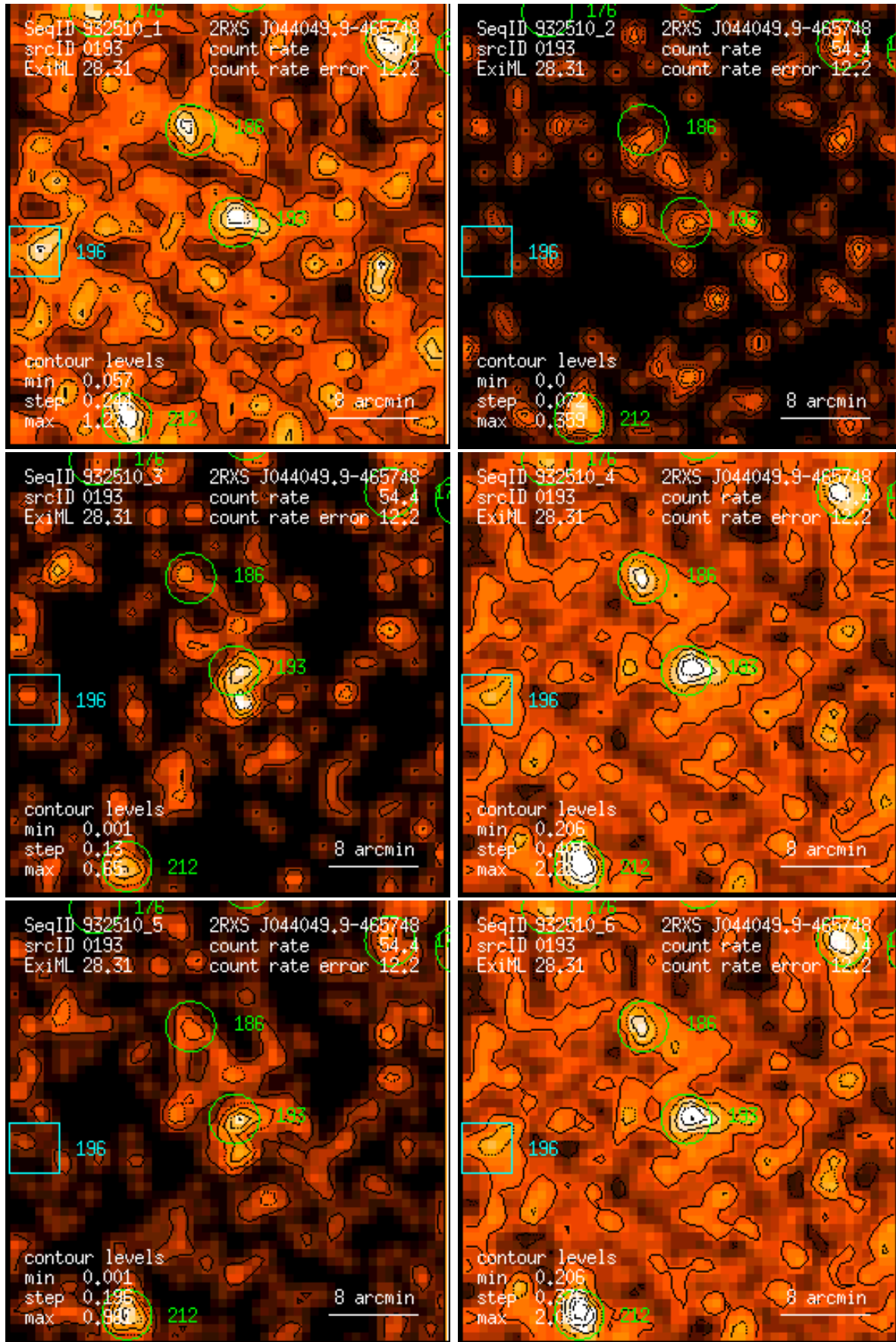
Figure 193: RASS 932510: detection 0193: band rate images, Gaussian filter: (1) PSPC channels 11 – 41, (2) 52 – 90, (3) 91 – 201, (4) 11 – 235, (5) 52 – 201, (6) 11 – 201. Broad band rates in counts/ks. Band rate contour levels in counts/ks/arcmin 2 .
