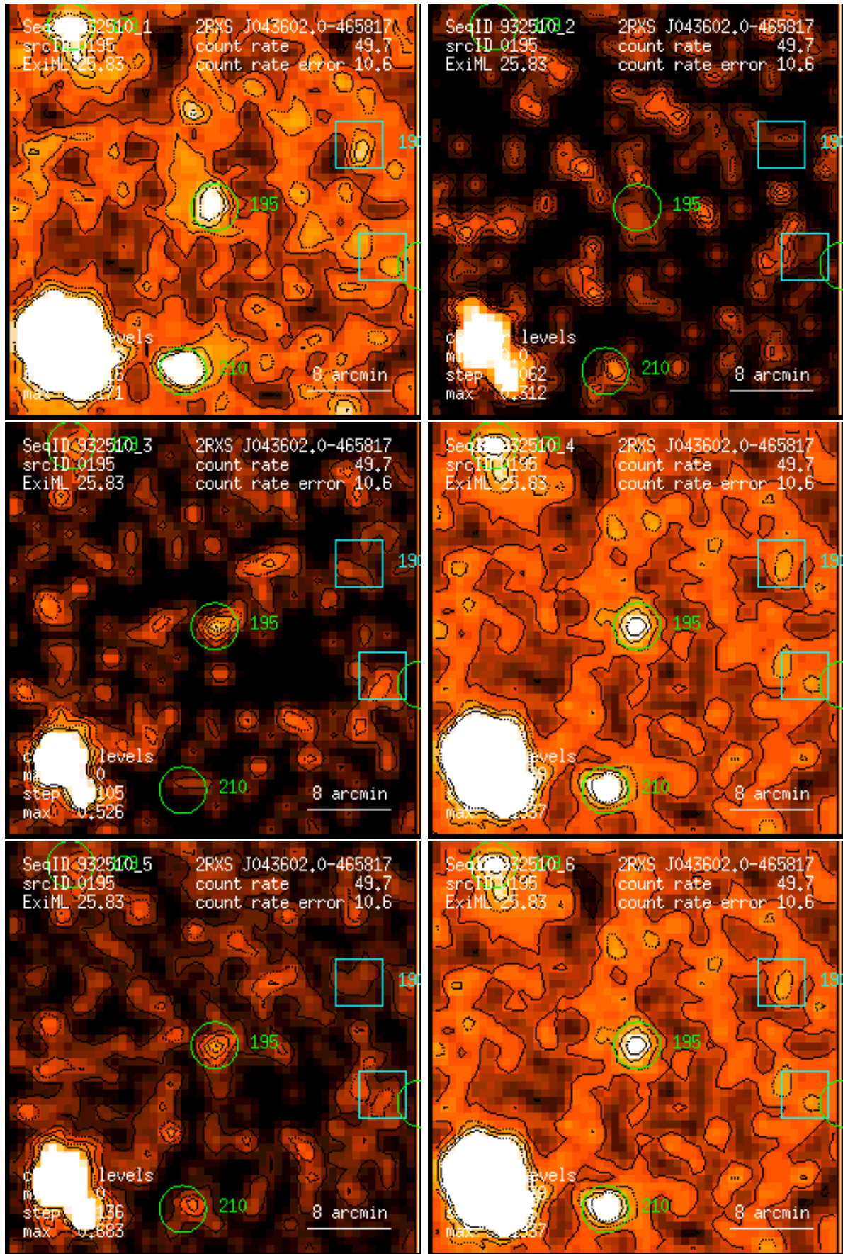
Figure 195: RASS 932510: detection 0195: band rate images, Gaussian filter: (1) PSPC channels 11 – 41, (2) 52 – 90, (3) 91 – 201, (4) 11 – 235, (5) 52 – 201, (6) 11 – 201. Broad band rates in counts/ks. Band rate contour levels in counts/ks/arcmin 2 .
