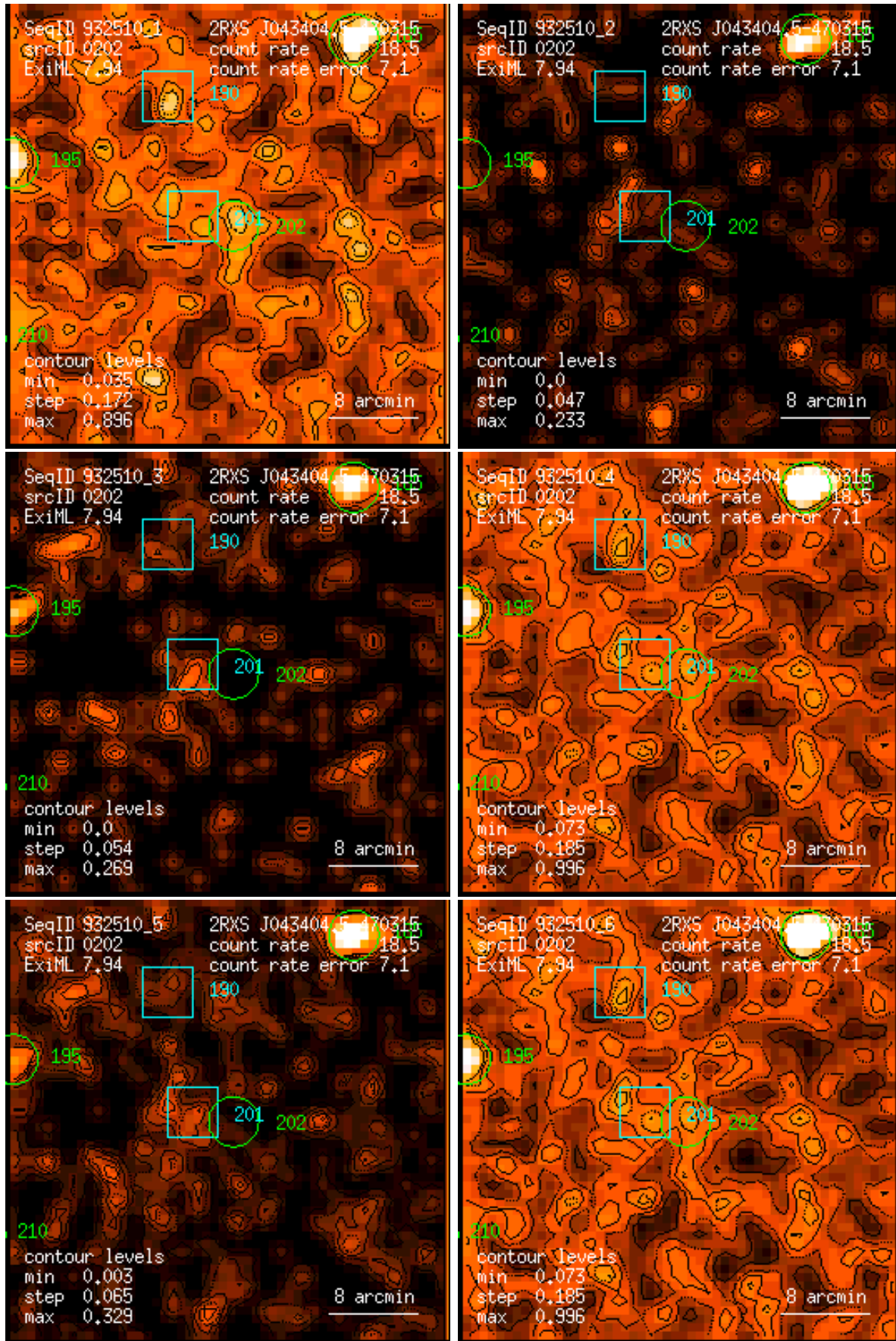
Figure 202: RASS 932510: detection 0202: band rate images, Gaussian filter: (1) PSPC channels 11 – 41, (2) 52 – 90, (3) 91 – 201, (4) 11 – 235, (5) 52 – 201, (6) 11 – 201. Broad band rates in counts/ks. Band rate contour levels in counts/ks/arcmin 2 .
