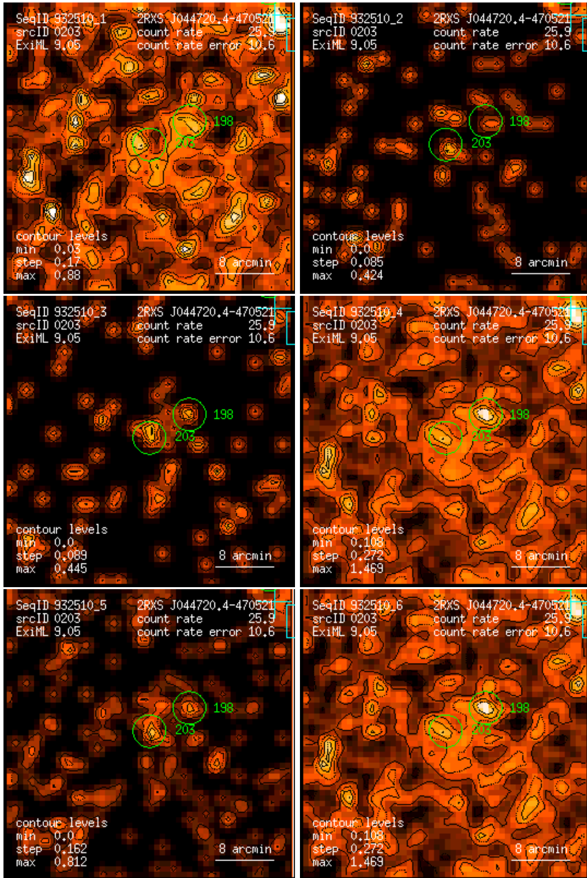
Figure 203: RASS 932510: detection 0203: band rate images, Gaussian filter: (1) PSPC channels 11 – 41, (2) 52 – 90, (3) 91 – 201, (4) 11 – 235, (5) 52 – 201, (6) 11 – 201. Broad band rates in counts/ks. Band rate contour levels in counts/ks/arcmin 2 .
