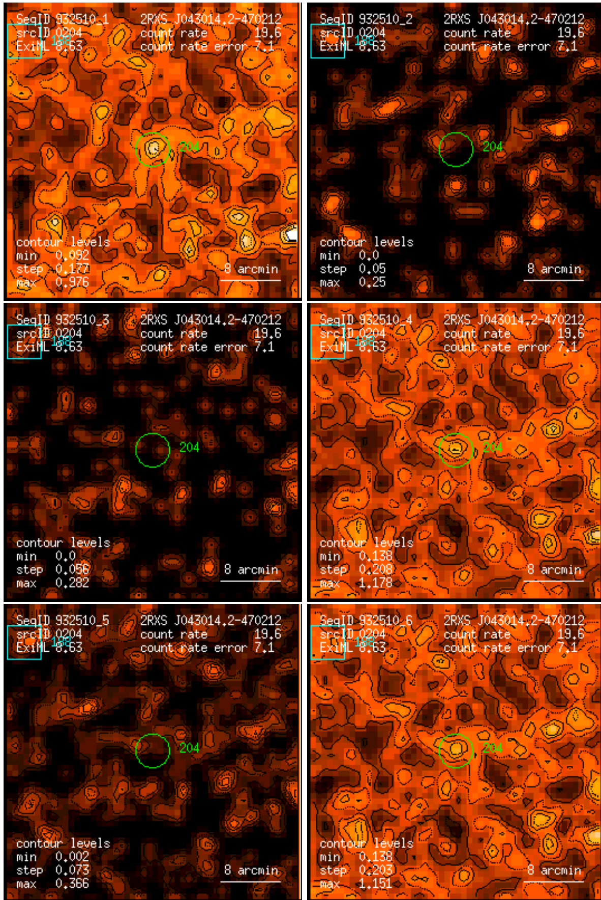
Figure 204: RASS 932510: detection 0204: band rate images, Gaussian filter: (1) PSPC channels 11 – 41, (2) 52 – 90, (3) 91 – 201, (4) 11 – 235, (5) 52 – 201, (6) 11 – 201. Broad band rates in counts/ks. Band rate contour levels in counts/ks/arcmin 2 .
