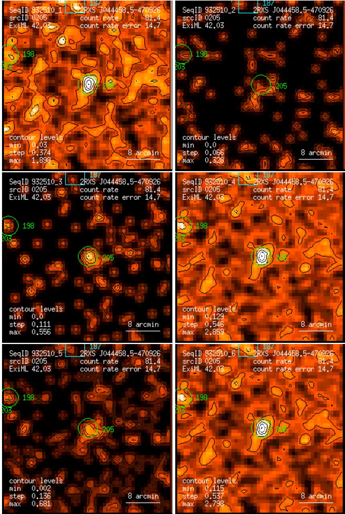
Figure 205: RASS 932510: detection 0205: band rate images, Gaussian filter: (1) PSPC channels 11 – 41, (2) 52 – 90, (3) 91 – 201, (4) 11 – 235, (5) 52 – 201, (6) 11 – 201. Broad band rates in counts/ks. Band rate contour levels in counts/ks/arcmin 2 .
