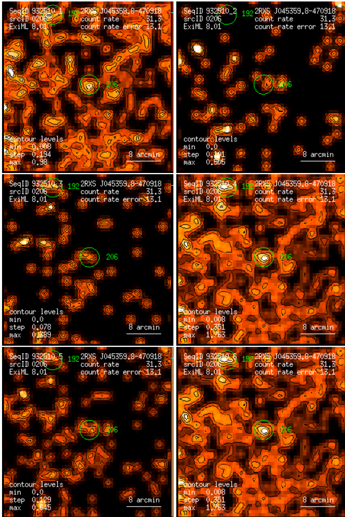
Figure 206: RASS 932510: detection 0206: band rate images, Gaussian filter: (1) PSPC channels 11 – 41, (2) 52 – 90, (3) 91 – 201, (4) 11 – 235, (5) 52 – 201, (6) 11 – 201. Broad band rates in counts/ks. Band rate contour levels in counts/ks/arcmin 2 .
