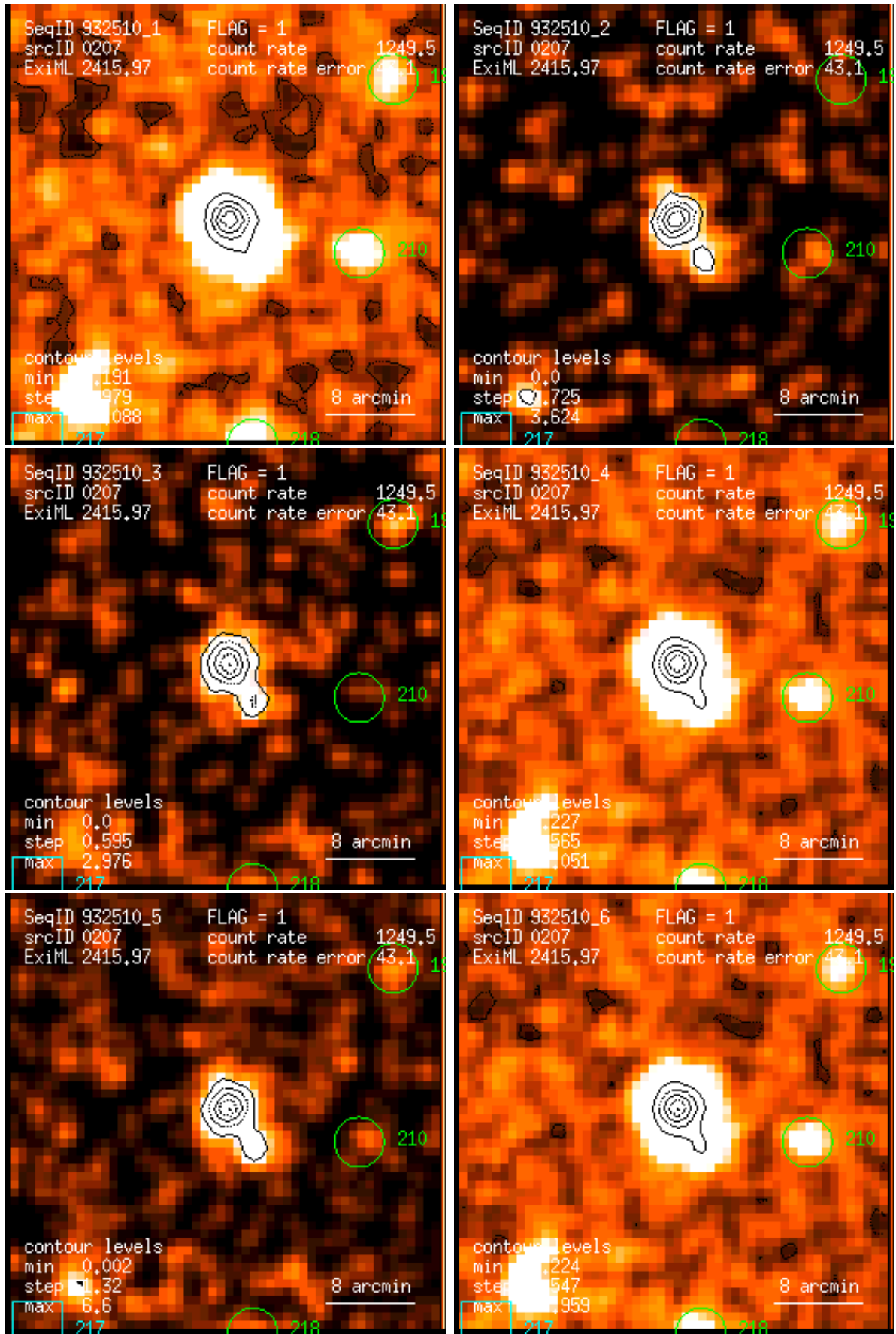
Figure 207: RASS 932510: detection 0207: band rate images, Gaussian filter: (1) PSPC channels 11 – 41, (2) 52 – 90, (3) 91 – 201, (4) 11 – 235, (5) 52 – 201, (6) 11 – 201. Broad band rates in counts/ks. Band rate contour levels in counts/ks/arcmin 2 .
