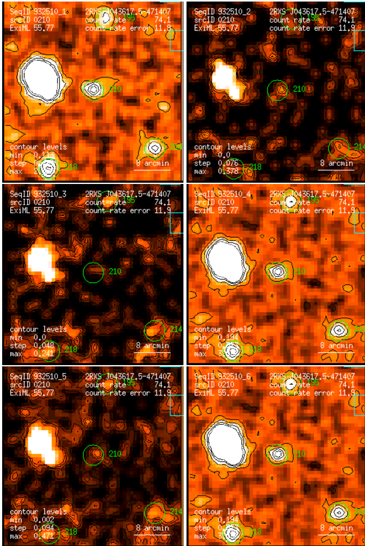
Figure 210: RASS 932510: detection 0210: band rate images, Gaussian filter: (1) PSPC channels 11 – 41, (2) 52 – 90, (3) 91 – 201, (4) 11 – 235, (5) 52 – 201, (6) 11 – 201. Broad band rates in counts/ks. Band rate contour levels in counts/ks/arcmin 2 .
