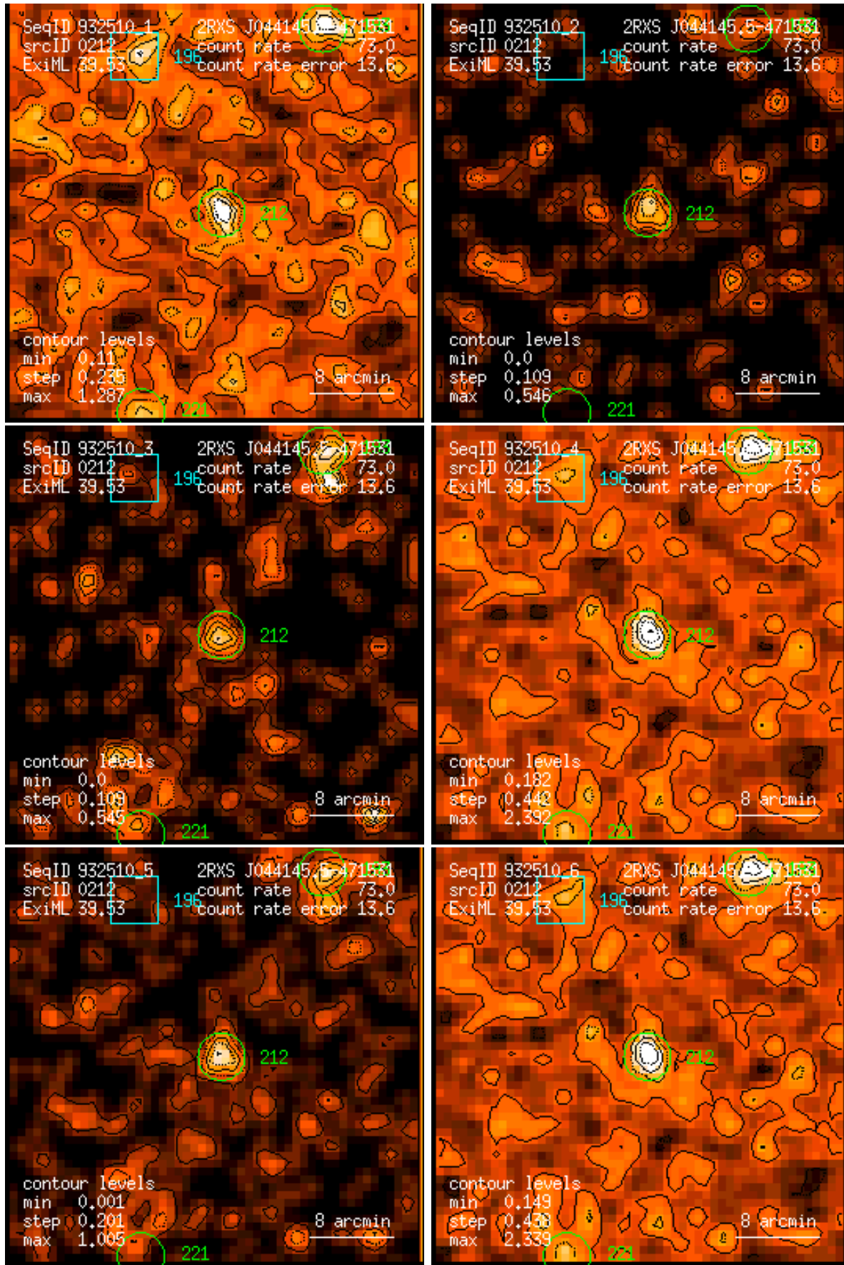
Figure 212: RASS 932510: detection 0212: band rate images, Gaussian filter: (1) PSPC channels 11 – 41, (2) 52 – 90, (3) 91 – 201, (4) 11 – 235, (5) 52 – 201, (6) 11 – 201. Broad band rates in counts/ks. Band rate contour levels in counts/ks/arcmin 2 .
