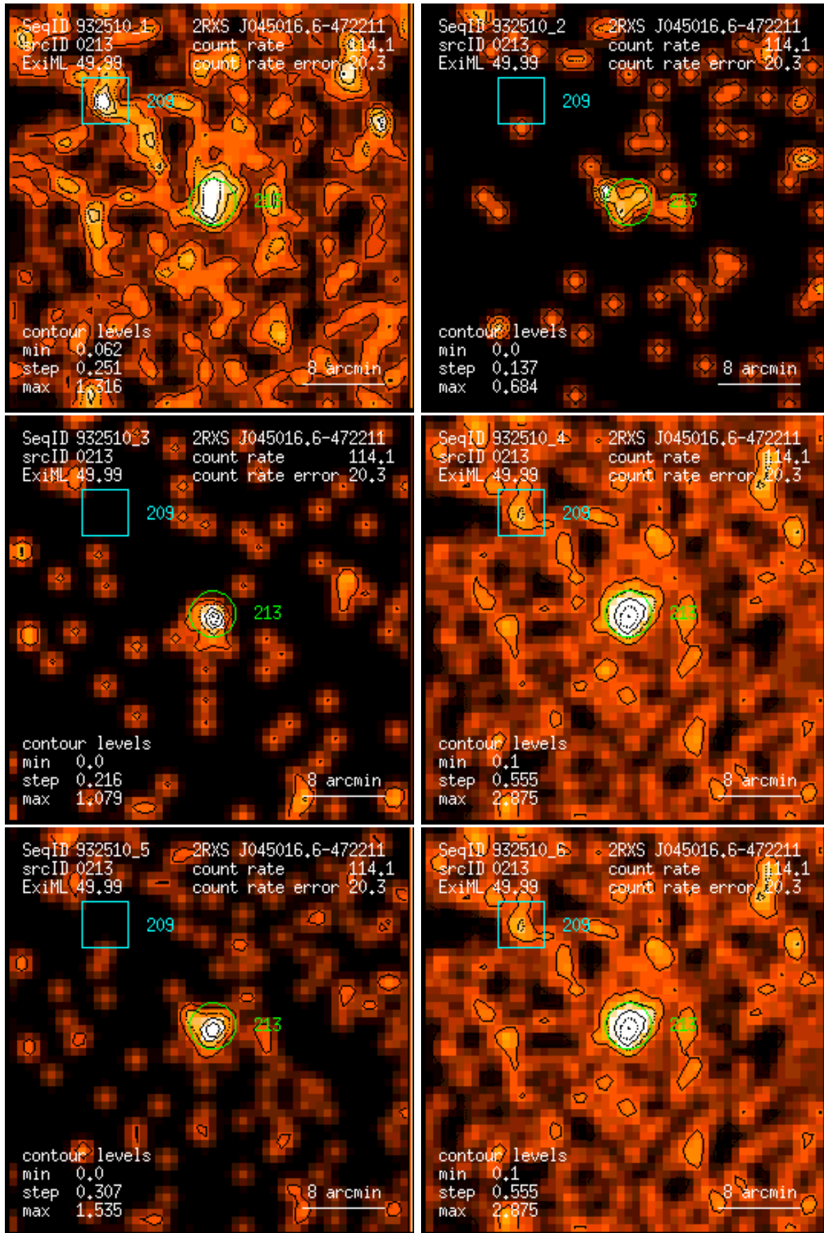
Figure 213: RASS 932510: detection 0213: band rate images, Gaussian filter: (1) PSPC channels 11 – 41, (2) 52 – 90, (3) 91 – 201, (4) 11 – 235, (5) 52 – 201, (6) 11 – 201. Broad band rates in counts/ks. Band rate contour levels in counts/ks/arcmin 2 .
