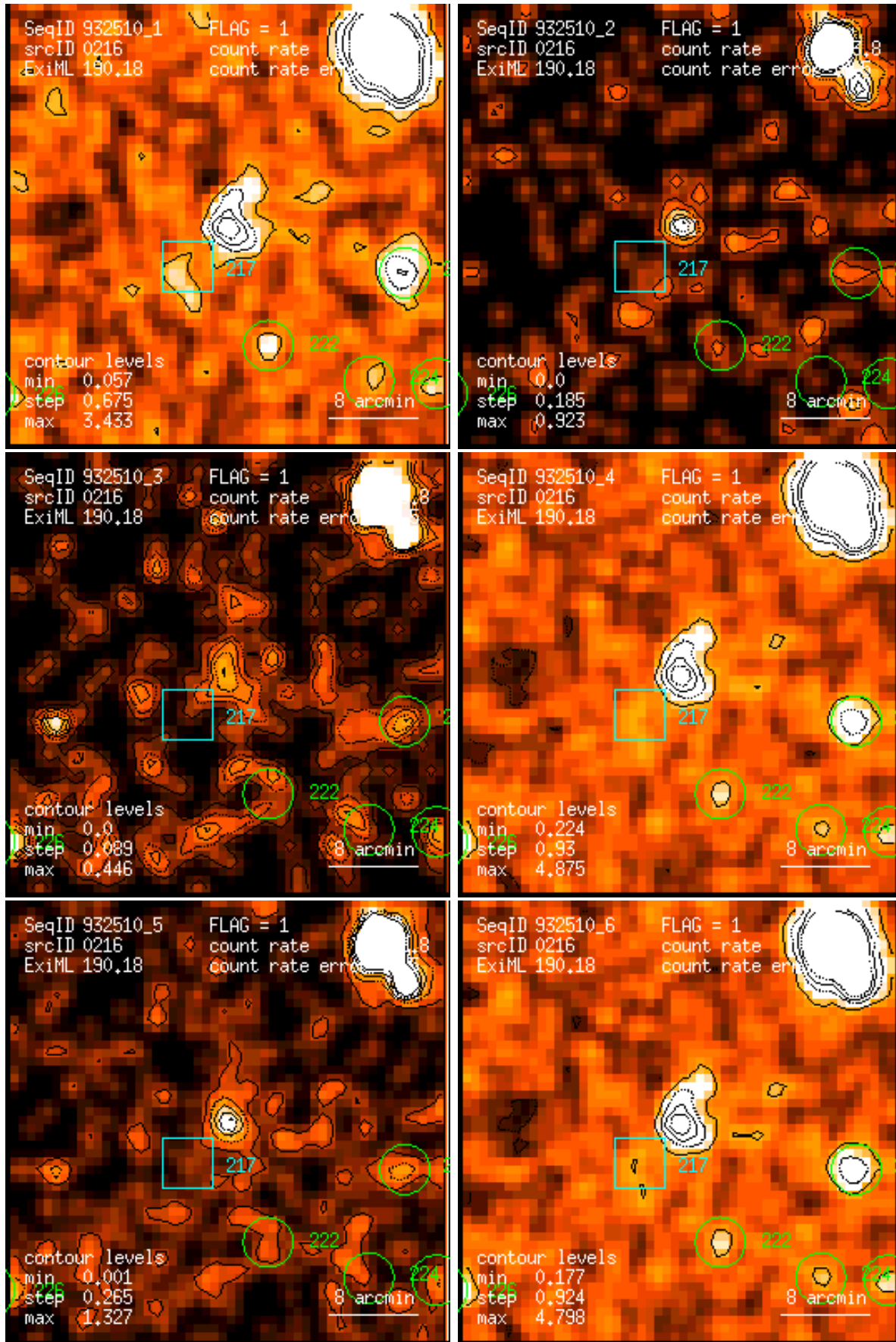
Figure 216: RASS 932510: detection 0216: band rate images, Gaussian filter: (1) PSPC channels 11 – 41, (2) 52 – 90, (3) 91 – 201, (4) 11 – 235, (5) 52 – 201, (6) 11 – 201. Broad band rates in counts/ks. Band rate contour levels in counts/ks/arcmin 2 .
