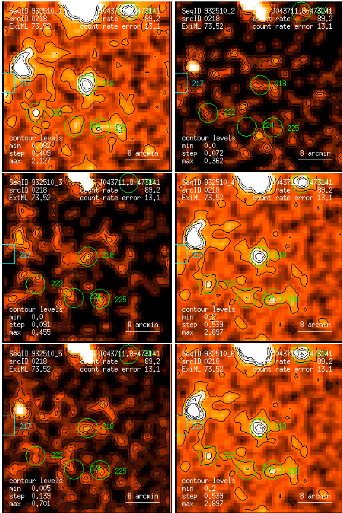
Figure 218: RASS 932510: detection 0218: band rate images, Gaussian filter: (1) PSPC channels 11 – 41, (2) 52 – 90, (3) 91 – 201, (4) 11 – 235, (5) 52 – 201, (6) 11 – 201. Broad band rates in counts/ks. Band rate contour levels in counts/ks/arcmin 2 .
